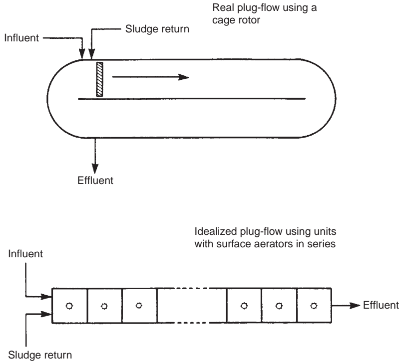
FIGURE 17.15 The oxidation ditch with a single rotor is close to the idealized design of a plug-flow reactor generally used in the treatment of wastewater.
