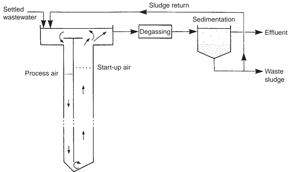
FIGURE 17.21 Schematic diagram of the deep shaft process developed by ICI plc employing a U-shaped reaction shaft.
