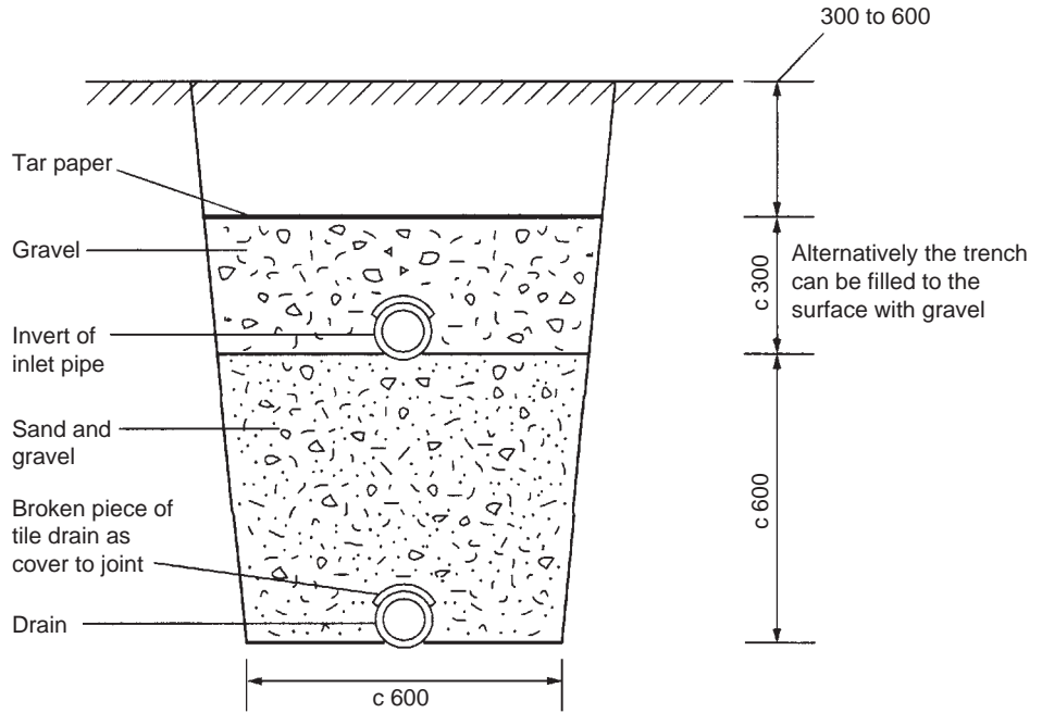
FIGURE 22.9 Cross-section of typical underdrain used in the UK. (Reproduced from British Standards Institution (1983) with permission of the British Standards Institution, London.)
