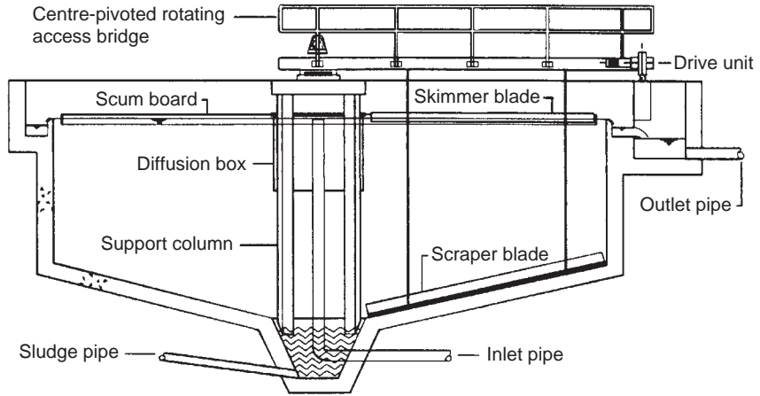
FIGURE 14.11 Radial-flow circular primary sedimentation tank. (Reproduced from Casey (1997) with permission of John Wiley and Sons Ltd, Chichester.)
