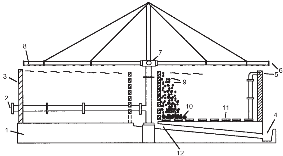
FIGURE 16.2 Basic constructional features of a conventional percolating filter: 1. foundation floor; 2. feed pipe; 3. retaining wall; 4. effluent channel; 5. ventilation pipe; 6. distributor arm; 7. rotary seal; 8. jets; 9. main bed of medium; 10. base layer of coarser medium; 11. drainage tiles; 12. central well for effluent collection. (Reproduced from Bruce and Hawkes (1983) with permission of Academic Press Ltd, London.)
