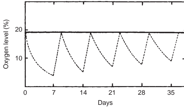
FIGURE 21.14 Cyclic variation of oxygen during composting within a pile that is periodically turned. The straight line represents the oxygen demand for a composting mass, and the dotted line the oxygen availability within the pile during each period between being turned. (Reproduced from Stentiford et al. (1985) with permission of Elsevier Science Ltd, London.)
