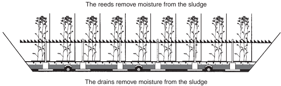
FIGURE 21.10 Design of a sludge mineralization reed bed.
