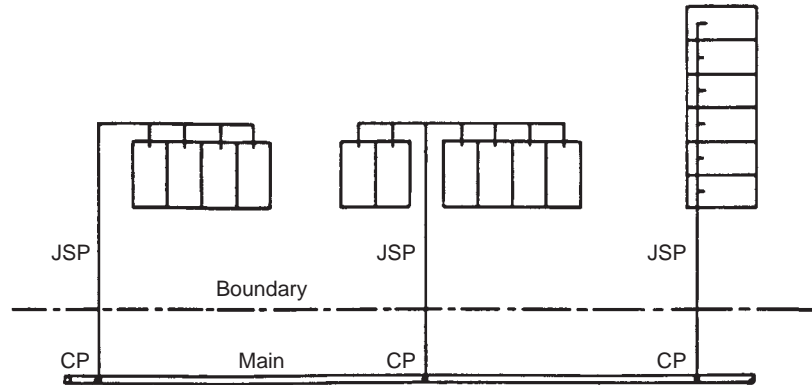
FIGURE 10.14 Examples of typical joint supply arrangements where CP is the communication pipe and JSP the joint supply pipe. (Reproduced from Latham (1990) with permission of the Chartered Institution of Water and Environmental Management, London.)
