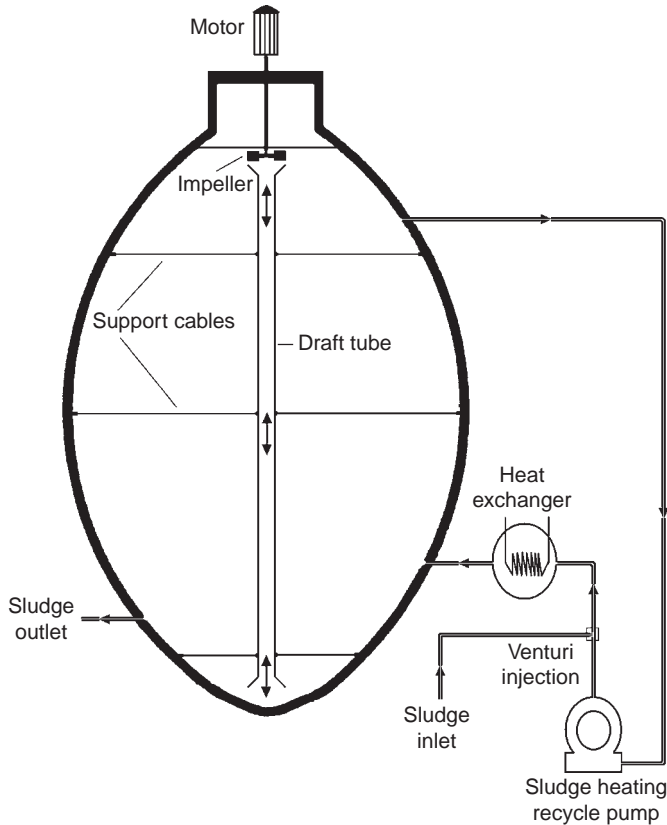
FIGURE 19.8 Design of modern egg-shaped anaerobic digester that prevents both settlement of solids and scum formation.
