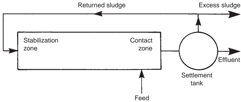
FIGURE 17.18 Schematic flow diagram of a single basin contact stabilization activated sludge system.
