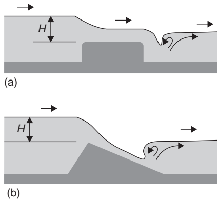
FIGURE 9.6 A schematic diagram showing the flow over (a) a broad crested weir and (b) a Crump weir.
