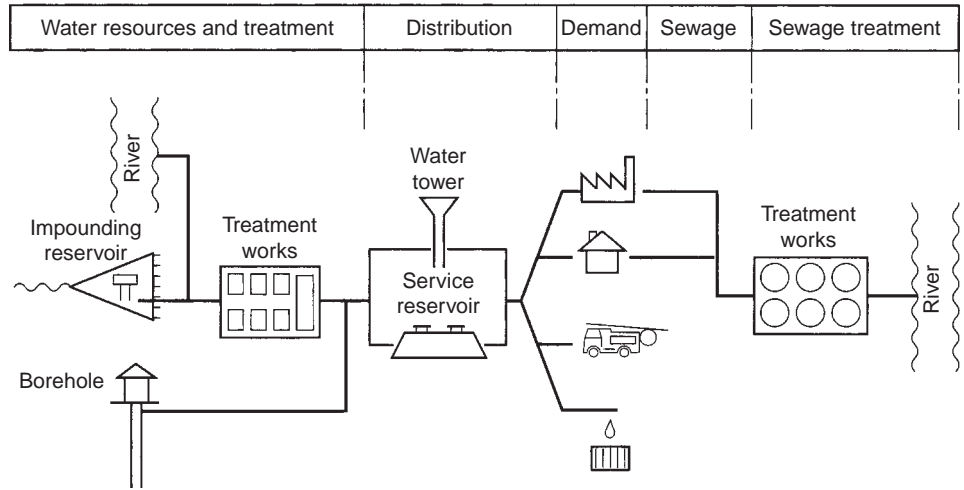
FIGURE 1.2 The water services cycle. Water is intercepted within the hydrological cycle for use and after treatment is returned back to the cycle. (Reproduced from Latham (1990) with permission of the Chartered Institution of Water and Environmental Management.)
