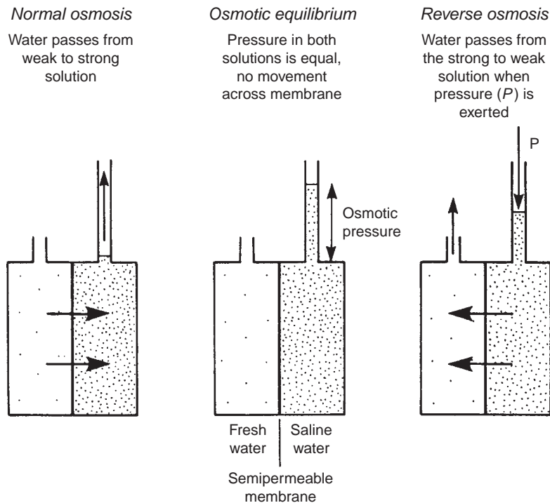
FIGURE 20.17 Principles of the RO process.
