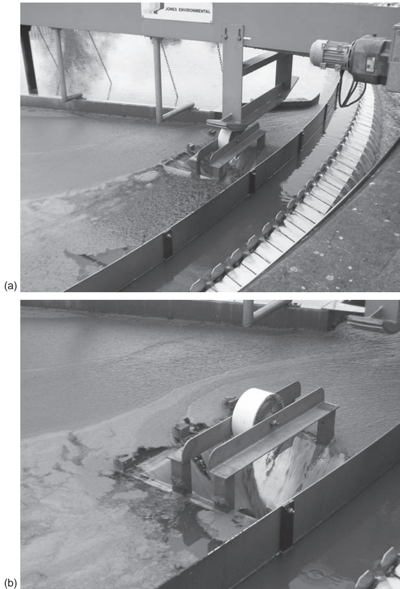
FIGURE 14.8 Surface scum removal for primary sedimentation. (a) As the skimming arm passes the spring supported scum box the sledge depresses the top of the box allowing the surface floating material to discharge into it. (b) Detail of box.
