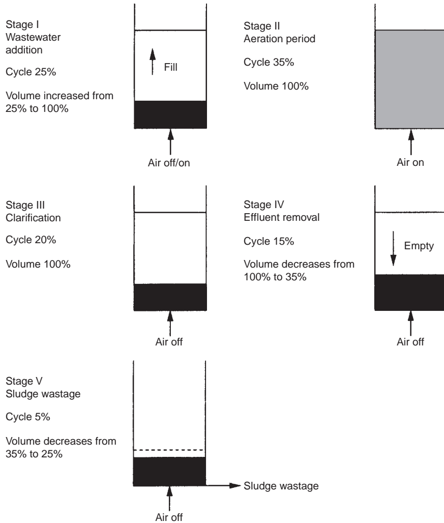
FIGURE 17.20 Typical cycle and configuration of an SBR.
