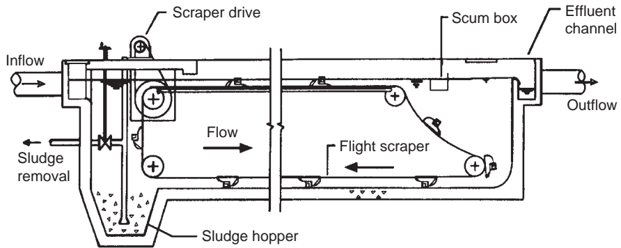
FIGURE 14.10 Horizontal-flow rectangular primary sedimentation tank. (Reproduced from Casey (1997) with permission of John Wiley and Sons Ltd, Chichester.)
