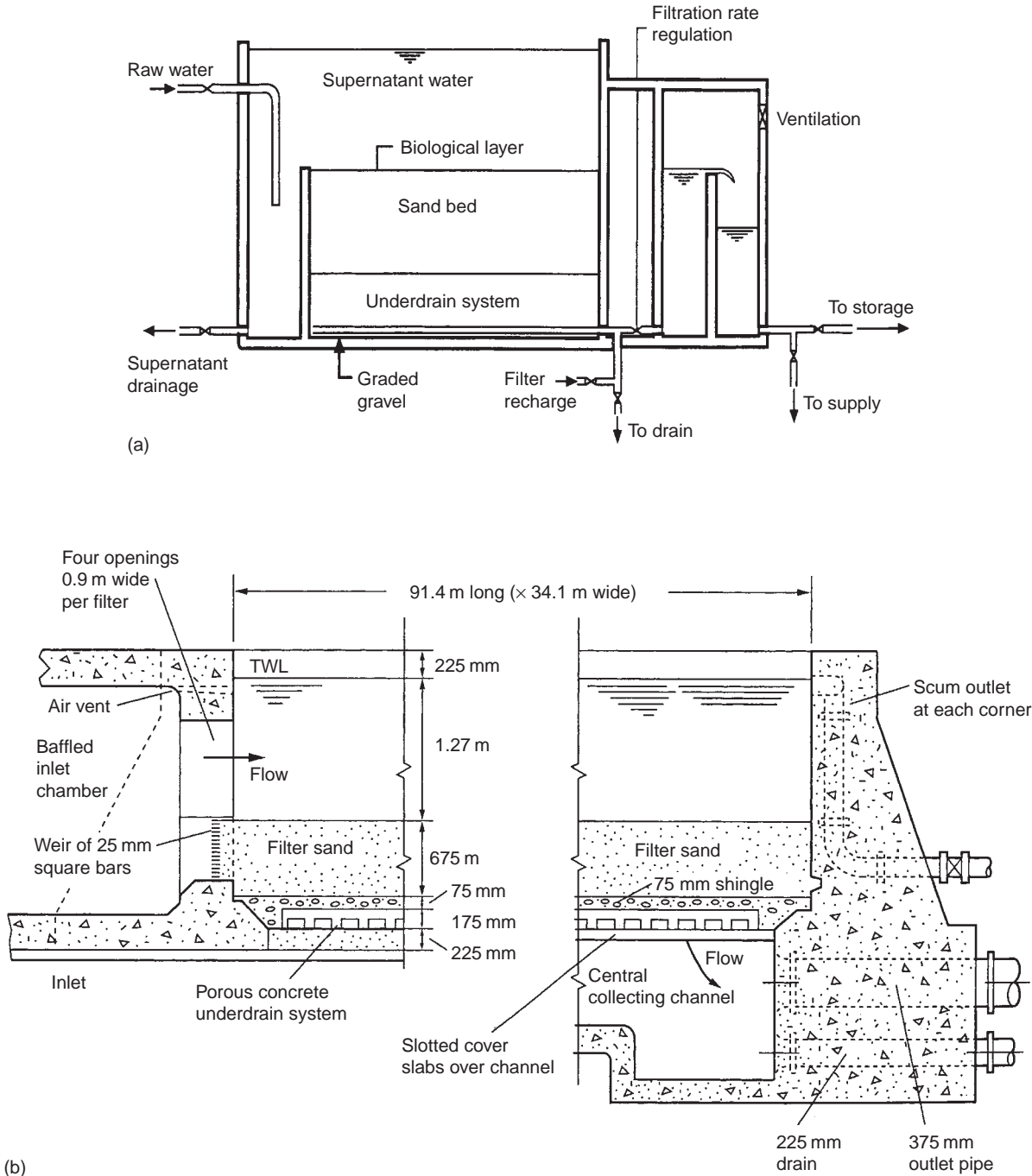
FIGURE 10.10 Schematic layout of a slow sand filter (a) showing constructional detail of typical filter (b). (Reproduced from (a) Casey (1997) with permission of John Wiley and Sons, Chichester and (b) Twort et al. (1994) with permission of Arnold, London.)
