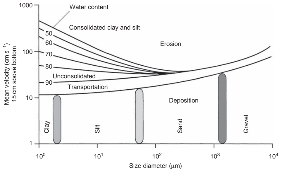
FIGURE 3.7 Velocity curves defining erosion, transport and deposition of sediments of differing grain size and water content. (Reproduced from Chapman (1996) with permission of UNESCO, Paris.)
