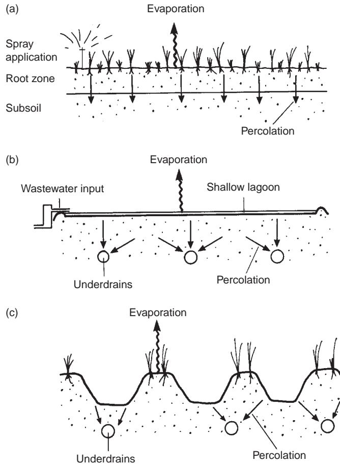
FIGURE 18.8 Land treatment by (a) surface irrigation, (b) flood irrigation, and (c) ridge and furrow irrigation.
