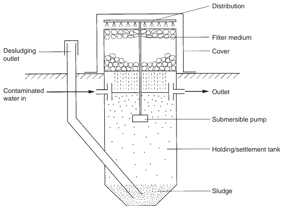
FIGURE 22.13 Schematic cross- section of the Biocler® complete wastewater treatment system for a single dwelling.
