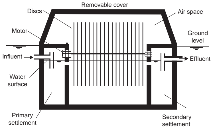
FIGURE 22.12 Schematic diagram of a rotating biological contactor used for single households.
