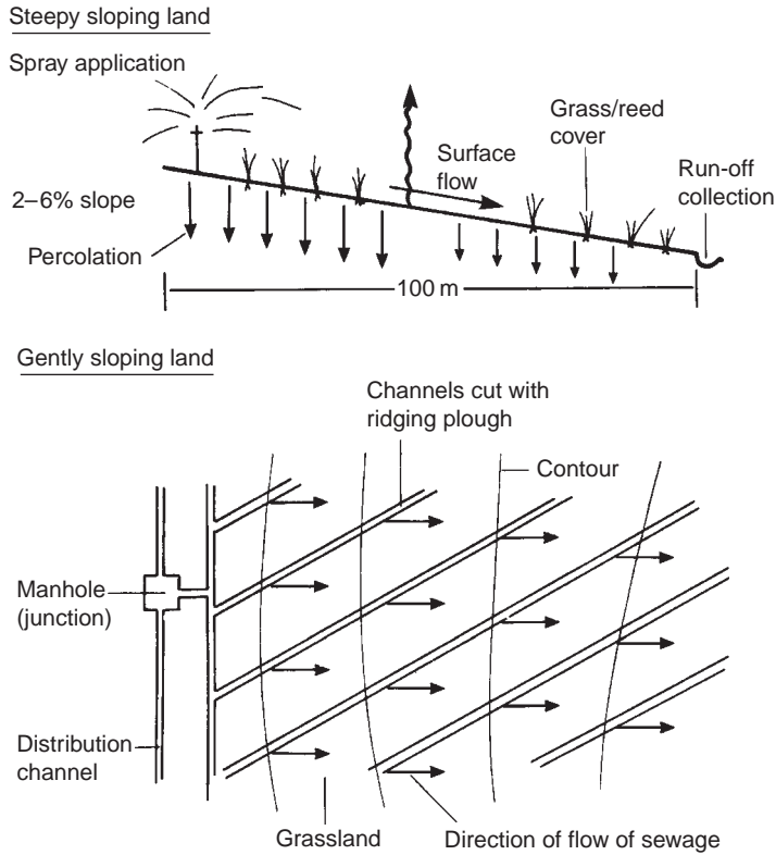
FIGURE 18.9 Land treatment by overland flow.
