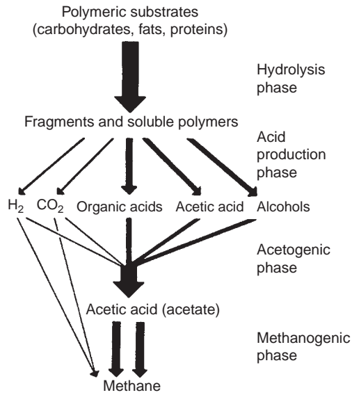
FIGURE 19.2 Major steps in anaerobic decomposition.
