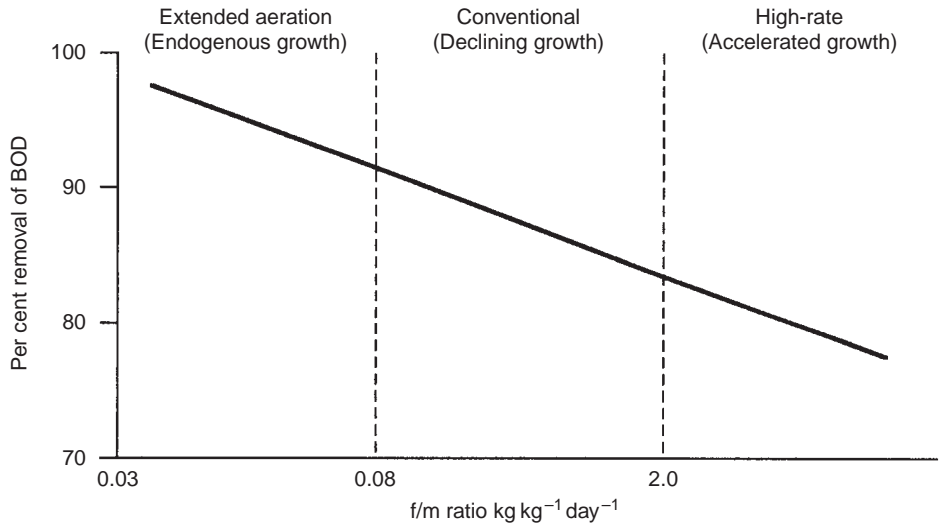
FIGURE 17.3 The relationship between f/m ratio and microbial growth.
