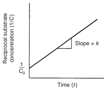
FIGURE 15.11 Arithmetical plot of a second-order reaction.
