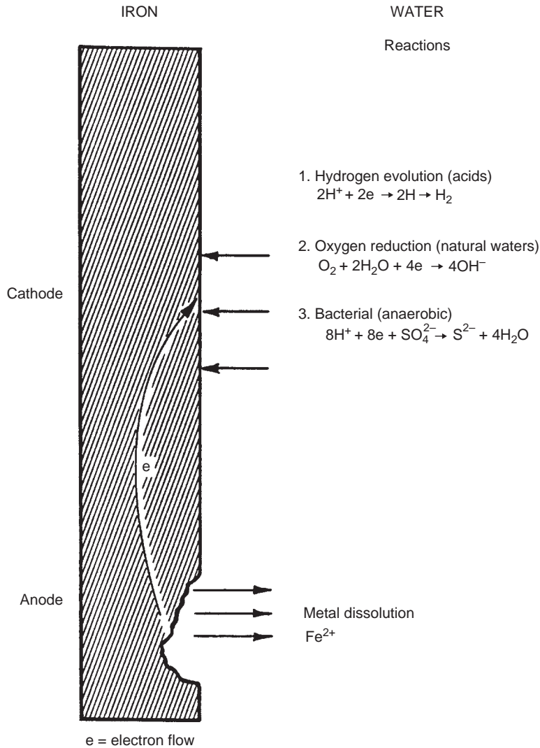
FIGURE 11.5 Main pathways leading to the corrosion of metal surfaces in household plumbing. (Reproduced from Ainsworth et al. (1981) with permission of WRc plc, Medmenham.)
