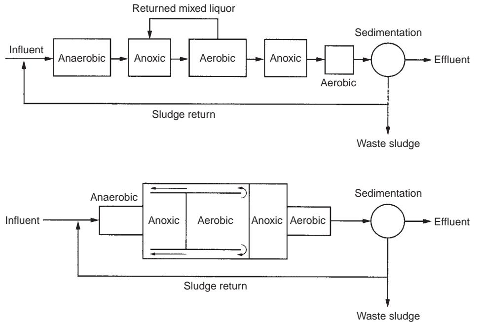
FIGURE 17.36 Typical schematic and plan design of the Bardenpho process.
