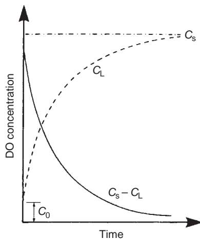
FIGURE 17.13 The relationship between the saturated DO concentration ( C_s ), the DO concentration at time zero ( C_0 ), the concentration at time t ( C_L ) and the DO deficit ( C_s - C_L ).
