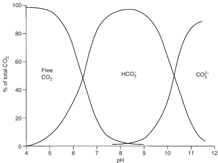
FIGURE 3.4 The relative proportions of different forms of inorganic carbon in relation to the pH of water under normal conditions. (Reproduced from Chapman (1996) with permission of UNESCO, Paris.)
