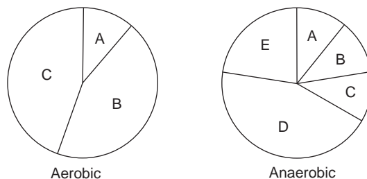
FIGURE 19.1 The proportion of the total energy in wastewater that is utilized under aerobic and anaerobic metabolism as: (A) lost heat energy; (B) respiration; (C) synthesis; (D) energy bound up in end products of metabolism; and (E) unused energy due to the lack of hydrogen acceptors.
