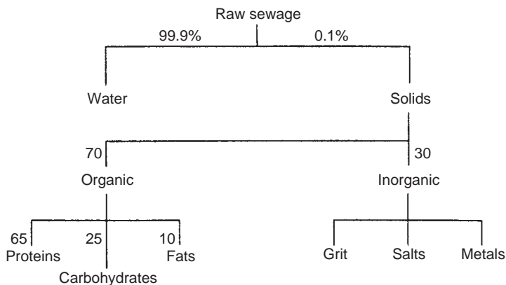
FIGURE 13.1 Composition of raw sewage. Components of solids fractions expressed as percentages.
