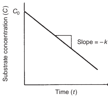
FIGURE 15.9 Arithmetical plot of a zero-order reaction.
