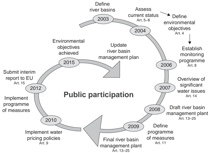
FIGURE 7.5 Key implementation steps of the WFD. (Reproduced with permission of the European Union, Brussels.)
