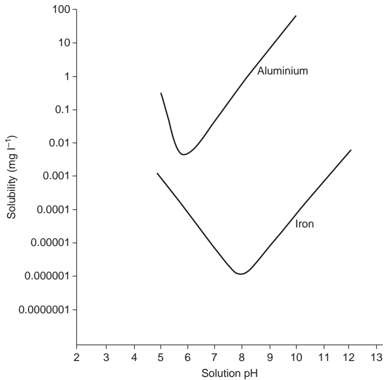
FIGURE 6.3 Solubility curves for aluminium and iron with pH.
