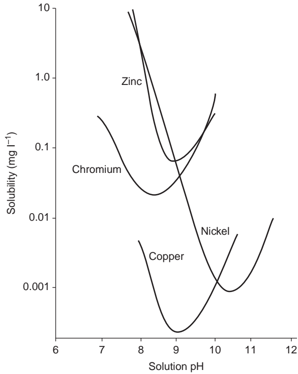
FIGURE 6.2 Solubility curves for common metals in freshwater with pH.
