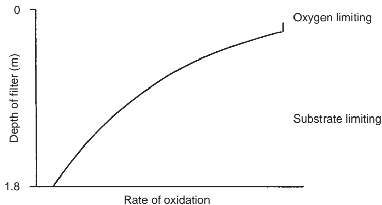
FIGURE 16.9 Rate of oxidation in relation to the depth of a percolating filter indicating where oxygen and substrate concentration are major limiting factors.
