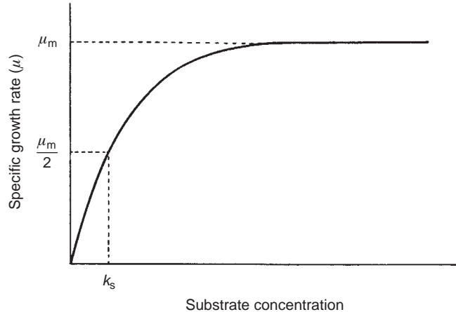
FIGURE 15.13 The relationship between specific growth rate and growth-limiting nutrient concentration.
