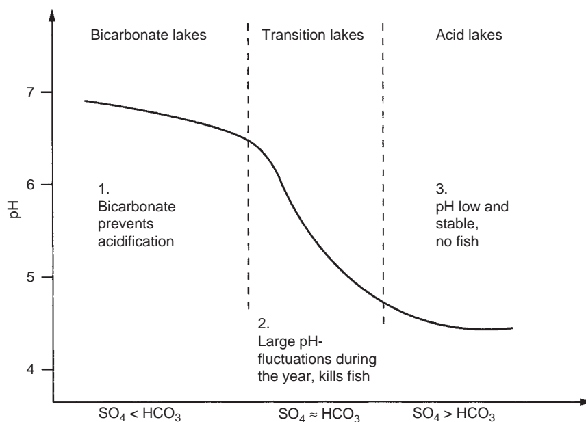
FIGURE 6.20 Classification of acidification of lakes using the ratio of sulphate to bicarbonate ions. (Reproduced from Mason (2002) with permission of Prentice Hall Ltd, London.)
