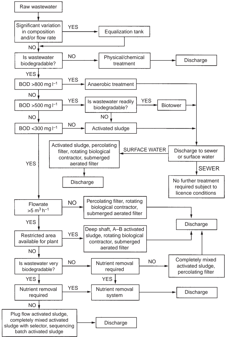
FIGURE 14.16 Process selection algorithm for biological wastewater treatment.
