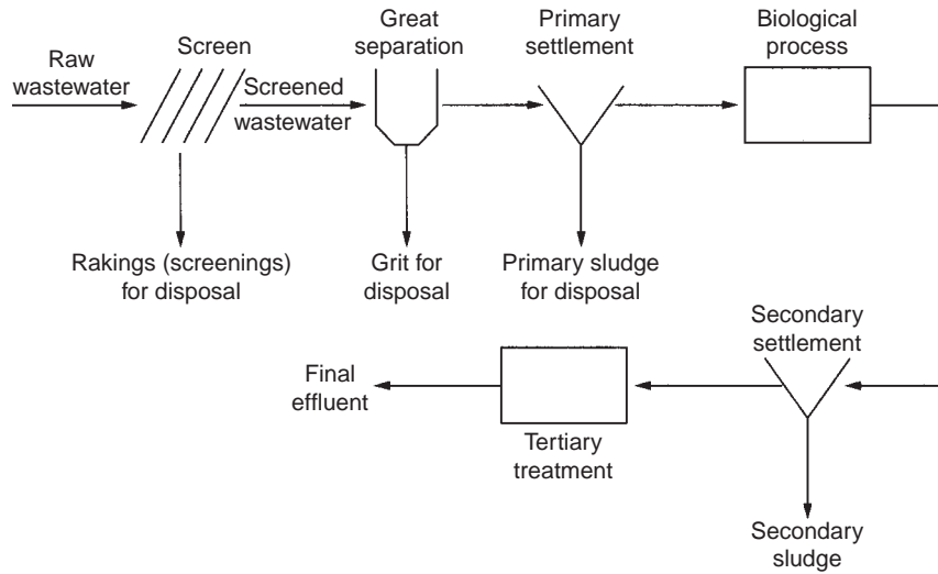
FIGURE 14.17 Typical layout of small sewage treatment plant serving a population of 20 000 or less.
