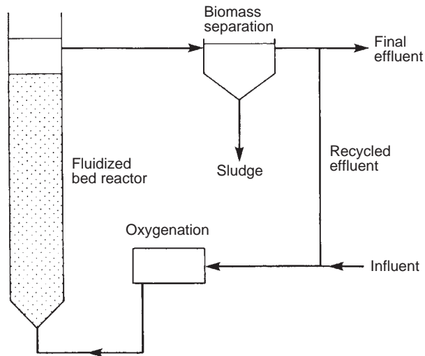
FIGURE 16.14 Typical design of fluidized bed reactor system.
