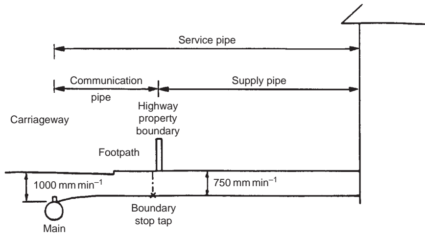
FIGURE 10.13 Arrangement of service pipes showing minimum depths to which pipes should be buried. (Reproduced from Latham (1990) with permission of the Chartered Institution of Water and Environmental Management, London.)
