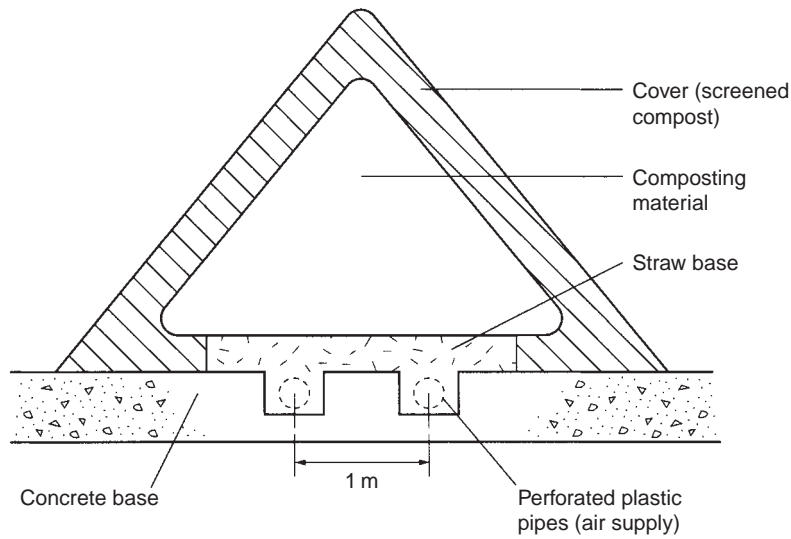
FIGURE 21.15 The most effective pile structure. (Reproduced from Stentiford et al. (1985) with permission of Elsevier Science Ltd, London.)
