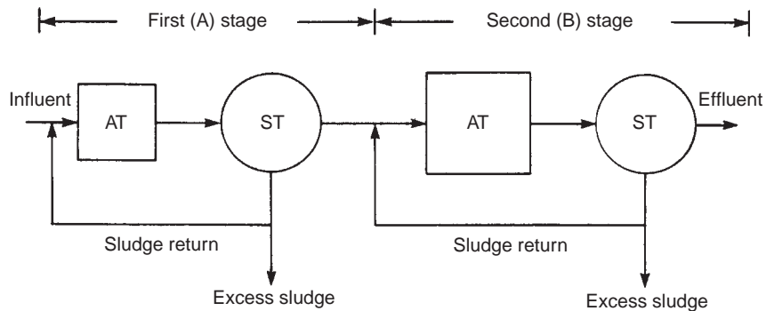
FIGURE 17.22 The A-B activated sludge process. AT: aeration tank; ST: sedimentation tank.
