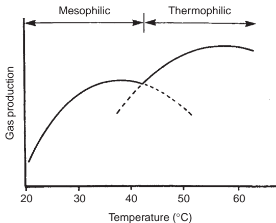
FIGURE 19.9 Effect of temperature on gas production.
