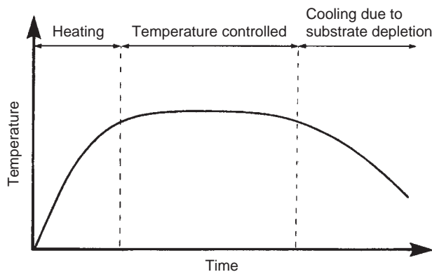
FIGURE 21.13 The three stages of the composting process in a static pile system. (Adapted from Stentiford et al. (1985) and reproduced with permission of Elsevier Science Ltd, London.)
