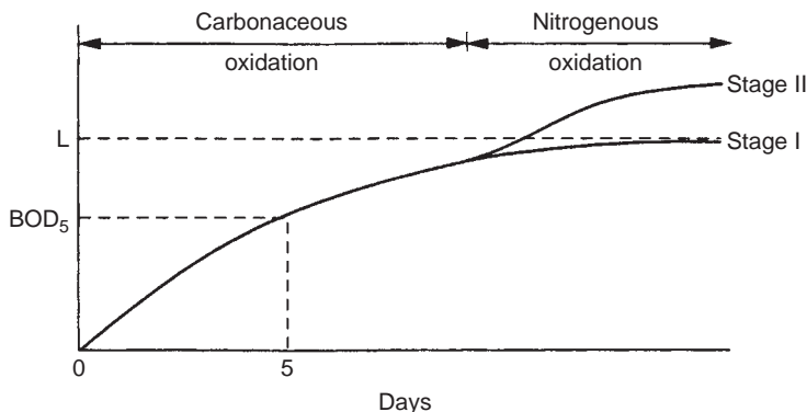
FIGURE 5.5 The typical BOD curve.
