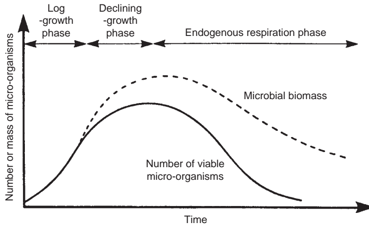
FIGURE 15.7 Microbial growth curves comparing total biomass and variable biomass.
