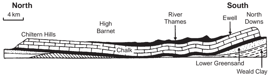
FIGURE 2.6 Cross-section through the London artesian basin. (Reproduced from Open University (1974) with permission of the Open University Press, Milton Keynes.)
