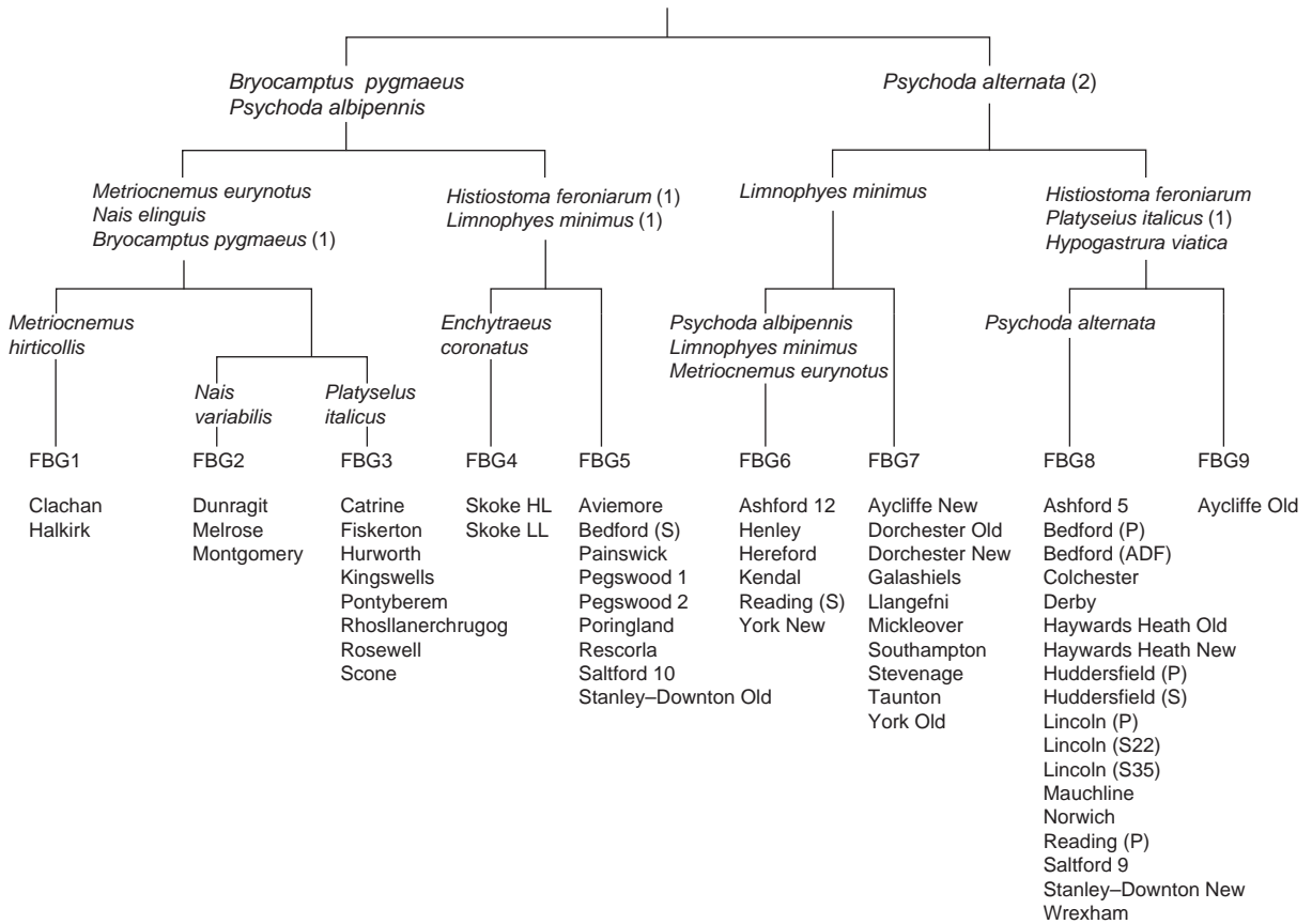
FIGURE 9.15 TWINSpan classification of the percolating filter beds based on macro-invertebrate species. The indicator species for various divisions are shown. The parentheses next to an indicator species denote abundance threshold: 1 = >1001^{-1} medium; 2 = >10001^{-1} medium. (Reproduced from Learner and Chawner (1998) with permission of the British Ecological Society, London.)
