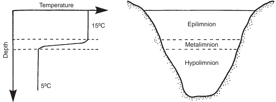
FIGURE 2.2 Thermal stratification in deep lakes and reservoirs.
