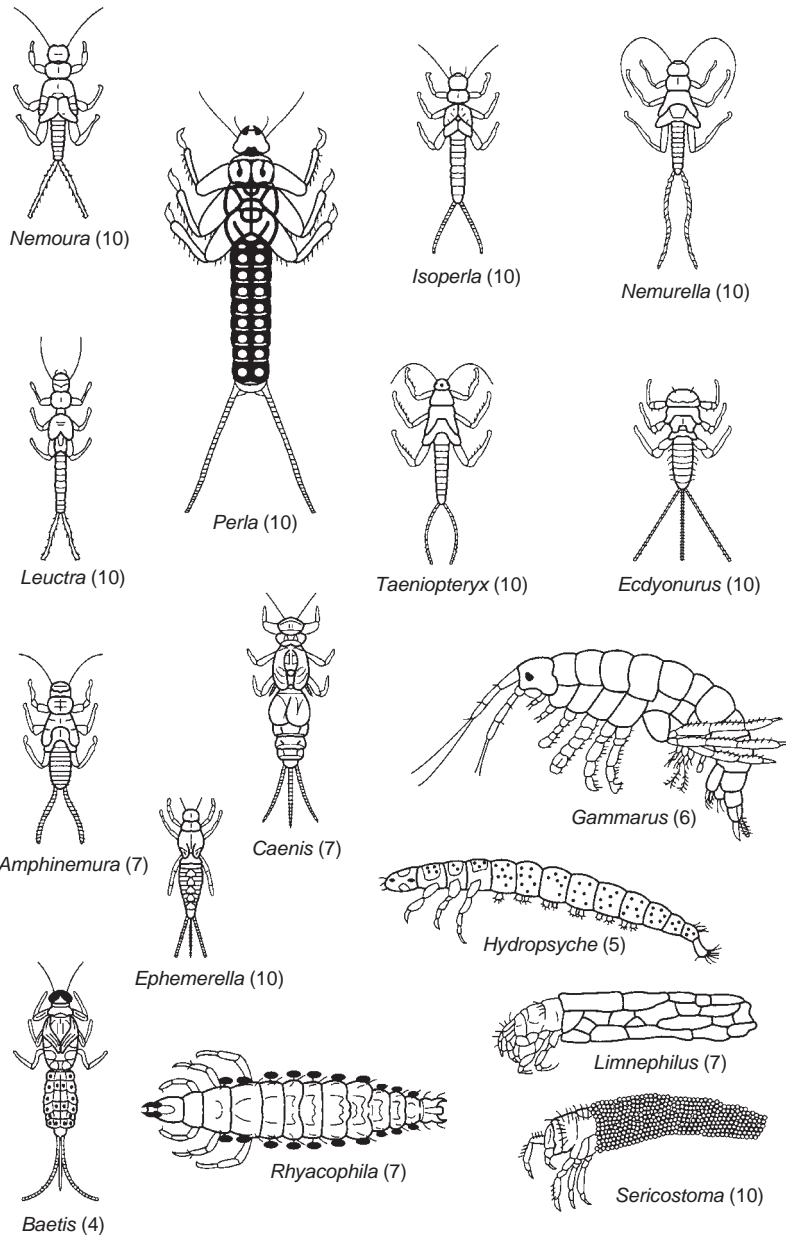
FIGURE 4.12 Macro-invertebrate species associated with erosional substrates. The Biological Monitoring Working Party (BMWP) score (Section 9.3) is given for each species in brackets. (Reproduced from Hellowell (1986) with permission of Kluwer Academic Publishers, Dordrecht, The Netherlands.)
