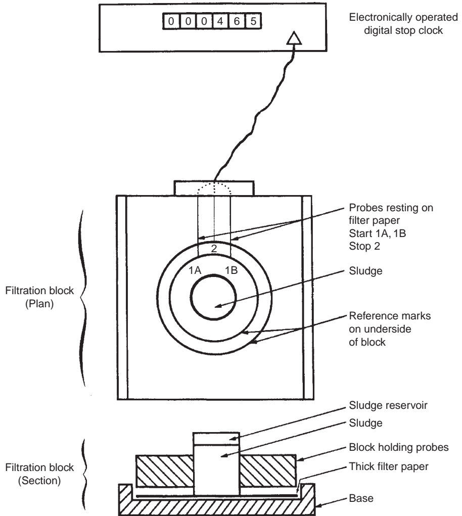
FIGURE 21.8 The capillary suction test (CST) apparatus. (Reproduced from the Department of the Environment (1985) with permission of Her Majesty's Stationery Office, London.)
