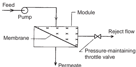
FIGURE 20.15 Schematic layout of a membrane filtration module. (Reproduced from Casey (1997) with permission of John Wiley and Sons Ltd, Chichester.)
