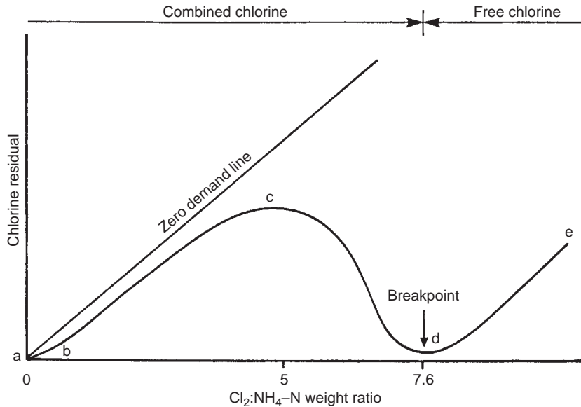
FIGURE 10.11 Breakpoint chlorination curve. See text for full explanation. (Reproduced from Gray (2008) with permission of Cambridge University Press, Cambridge.)
