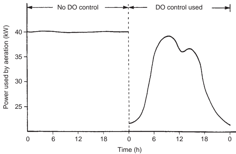
FIGURE 17.12 The effect on power consumption by aerators in an oxidation ditch when dissolved oxygen (DO) control is used.
