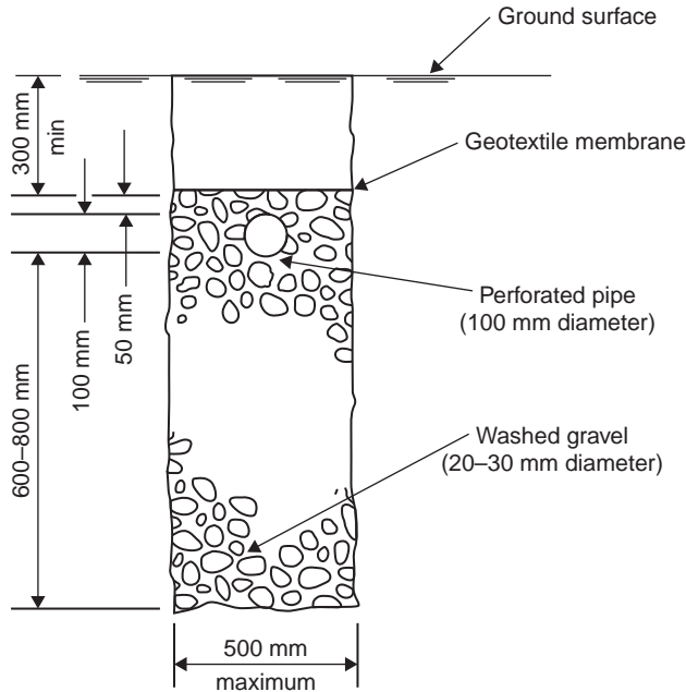
FIGURE 22.7 Cross-section through a standard percolation trench.
