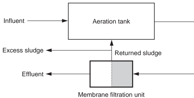
FIGURE 20.21 MBR system employing an external membrane filtration unit.
