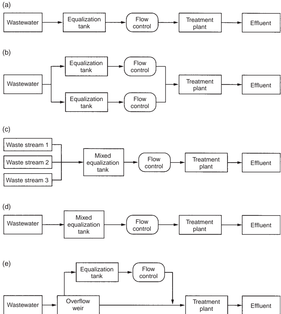
FIGURE 20.1 Major process configurations of equalization tanks. Wastewater must undergo screening and grit removal, if necessary, before equalization. (a) In-line system; (b) alternating in-line system; (c) completely mixed combined system; (d) in-line completely mixed system; (e) sidestream system.
