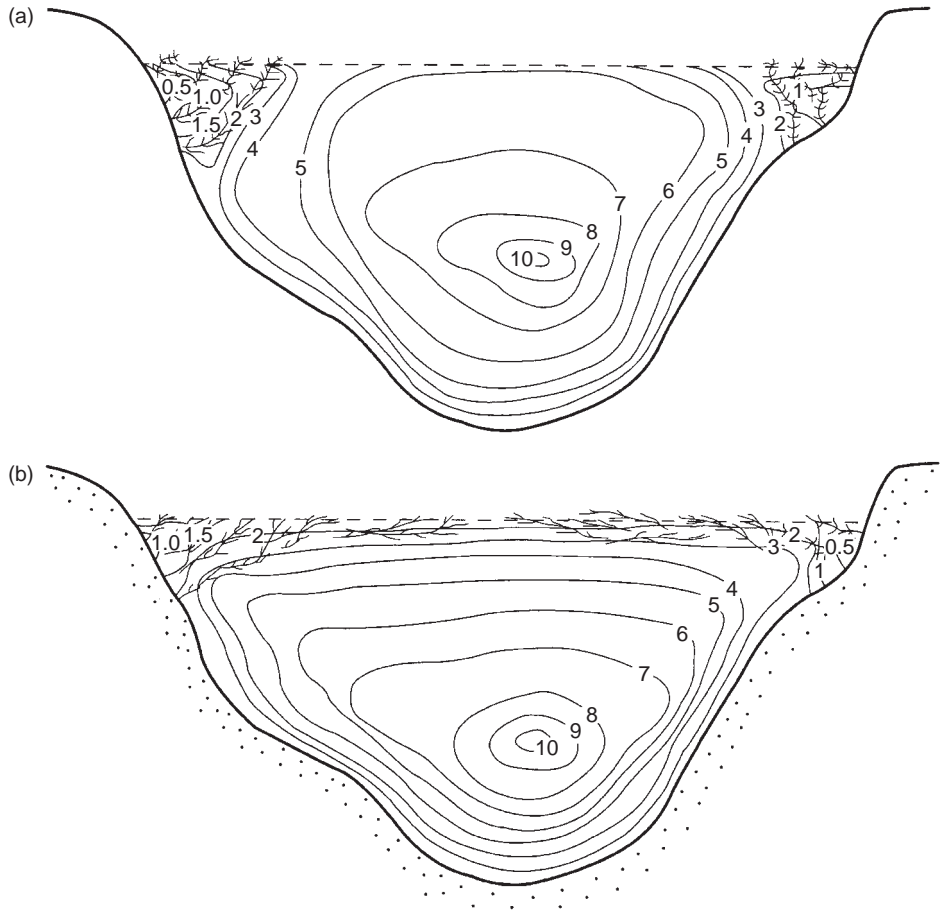
FIGURE 3.2 Transverse section through a small river channel. Contours of equal velocity are in \text{cm s}^{-1} . (a) Macrophytes limited to the banks only and (b) extending over the entire surface.
