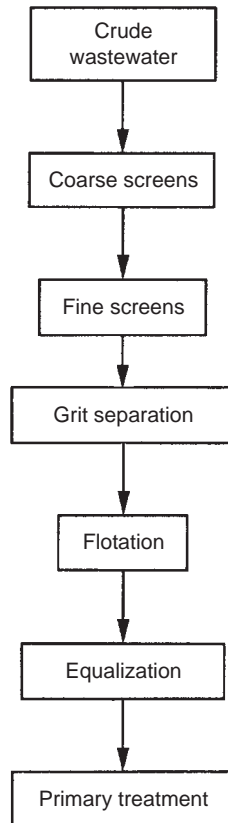
FIGURE 14.2 Summary of preliminary wastewater treatment processes.
