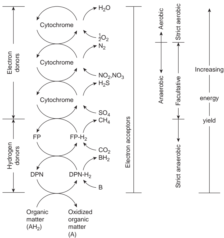
FIGURE 15.5 Dehydrogenation of wastewater showing relative energy yields for various ultimate electron acceptors.
