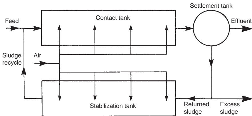
FIGURE 17.17 Schematic flow diagram of a contact stabilization activated sludge system.
