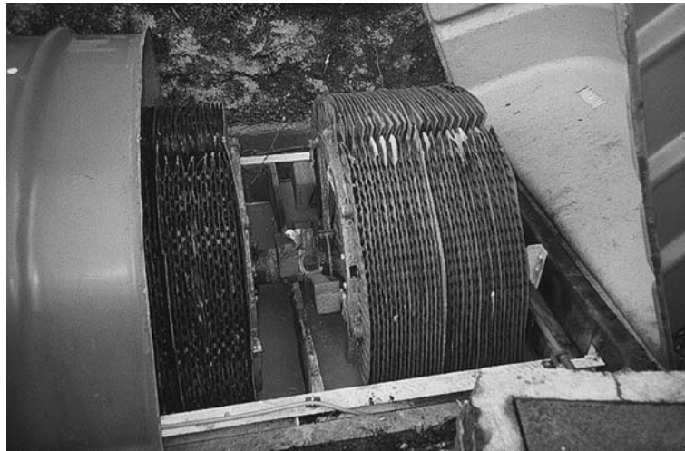
FIGURE 16.11 A small rotating biological contractor treating the waste from a small hotel. The plastic covers have been lifted to expose the plastic discs on which the biomass grows.
