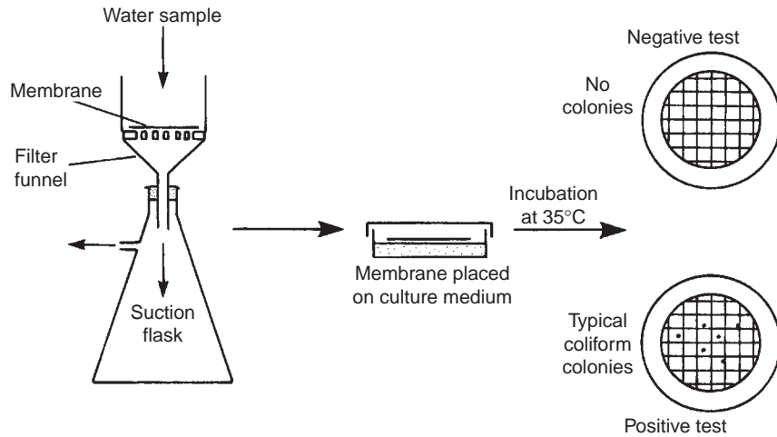
FIGURE 12.3 Major steps in coliform testing by the membrane filtration technique.
