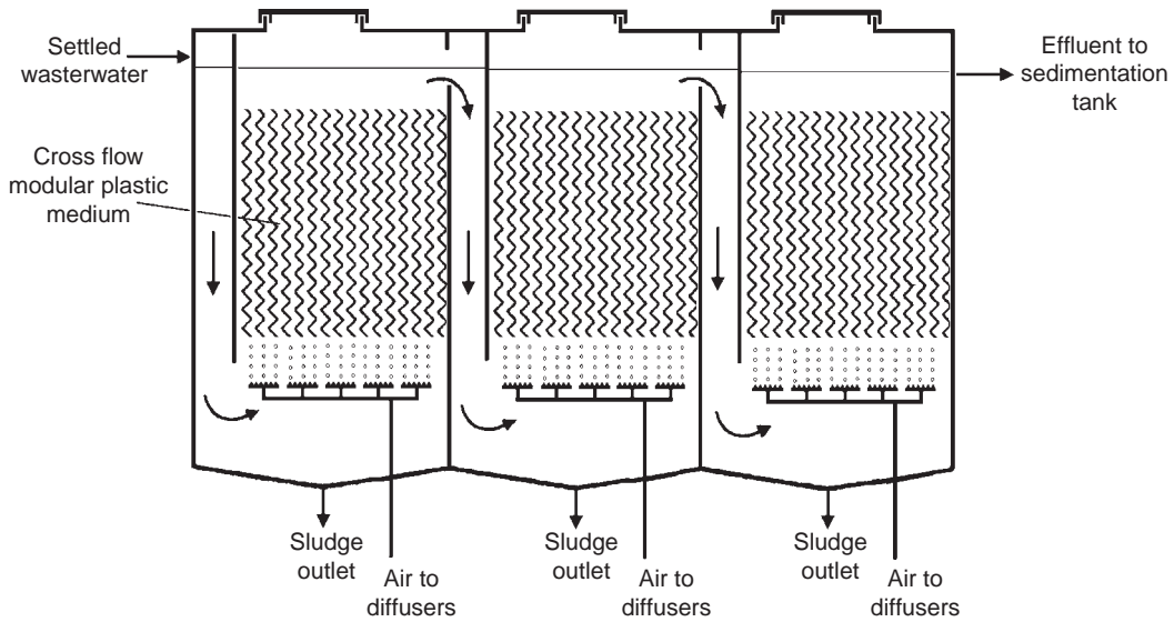
FIGURE 16.13 Schematic diagram of submerged aerated filters in series.
