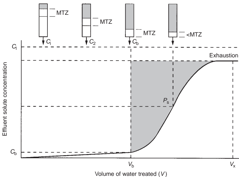
FIGURE 20.11 Typical breakthrough curve for activated carbon showing movement of the MTZ with the throughput volume. (Reproduced from Metcalf and Eddy (1991) with permission of McGraw-Hill Inc., New York.)
