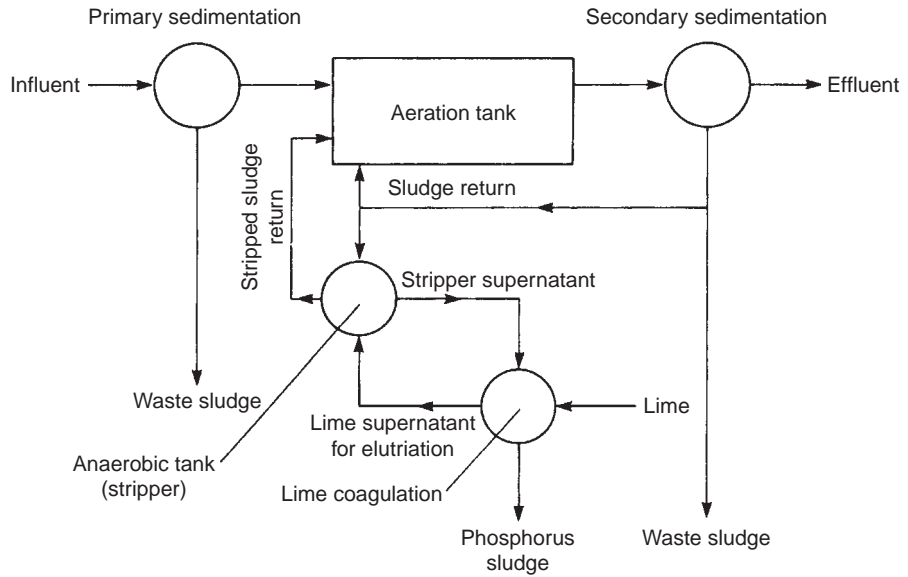
FIGURE 17.35 The phostrip process.
