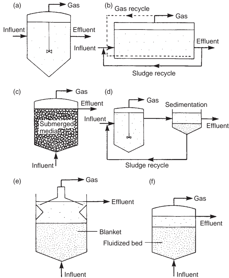
FIGURE 19.3 Schematic representation of digester types. Flow-through digesters (a and b) and contact systems (c–f). See text for details.
