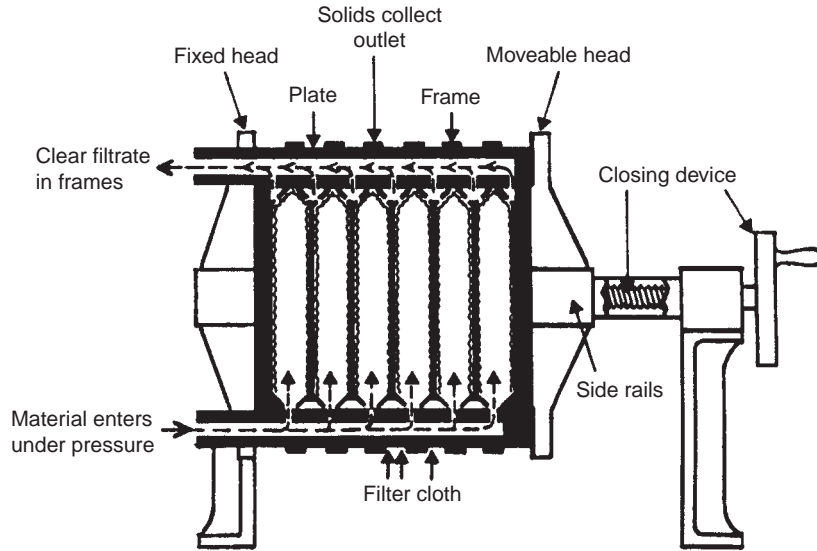
FIGURE 21.7 Sludge filter press. (Reproduced from Casey and O'Connor (1980) with permission of Enterprise Ireland, Dublin.)
