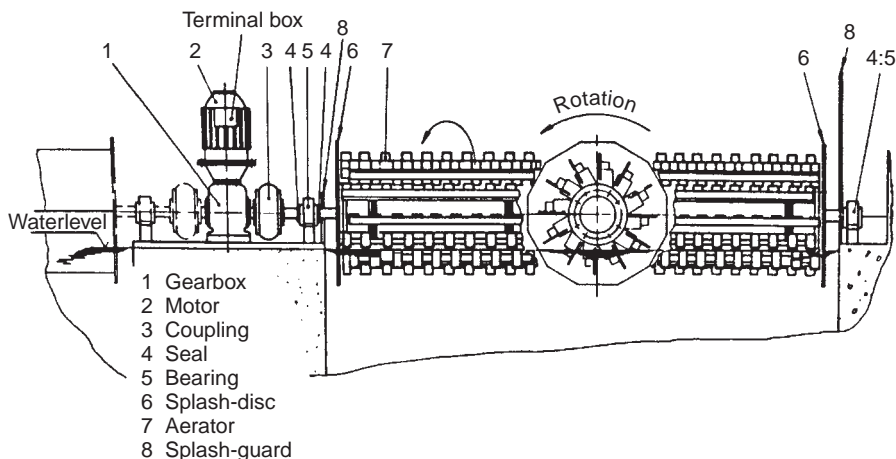
FIGURE 17.7 General arrangement of a Mammoth horizontal rotor.
