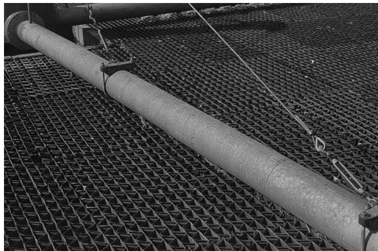
FIGURE 16.8 Modular plastic medium is used for high-rate applications or for treating strong wastewaters.
