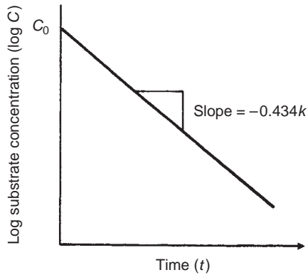
FIGURE 15.10 Semi-log plot of a first-order reaction.
