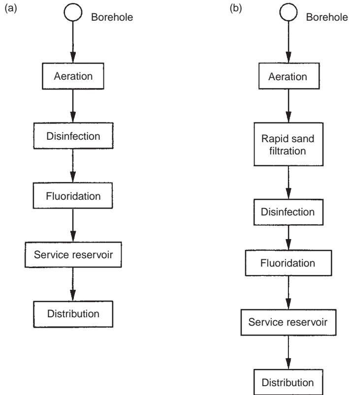
FIGURE 10.1 Sequence of treatment for groundwater sources (a) of excellent quality and (b) with moderate concentrations of iron.
