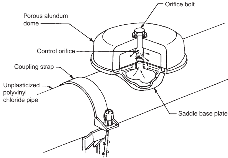
FIGURE 17.9 Dome diffuser. (Reproduced from IWPC (1987) with permission of the Chartered Institution of Water and Environmental Management, London.)
