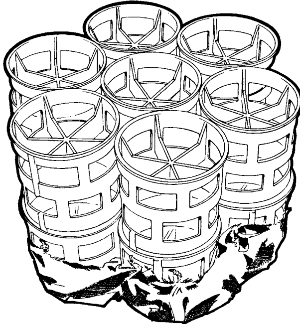
FIGURE 9.10 The UK standard colonization unit used as an artificial substrate for macro-invertebrates in river sites not suitable for sampling with either a hand-net or Surber sampler. (Reproduced from Department of the Environment (1983b) with permission of Her Majesty's Stationery Office, London.)
