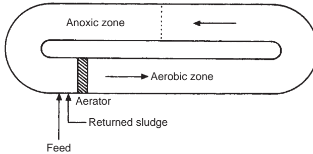
FIGURE 17.33 Aerobic and anoxic zone for dual nitrification – denitrification within single oxidation ditches.
