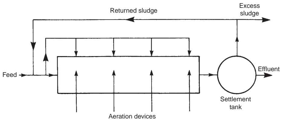
FIGURE 17.19 Schematic flow diagram of step aeration in a conventional plug-flow activated sludge system.
