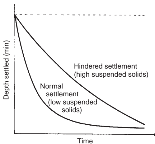
FIGURE 20.7 Comparison of the rate of settlement of solids for a wastewater with a high suspended solids concentration showing hindered settlement compared with a normal wastewater containing a low suspended solids concentration.
