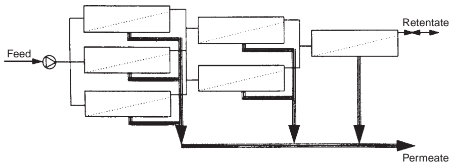
FIGURE 20.18 Schematic diagram of the arrangement of modules in a taper plant. (Reproduced from Scott and Hughes (1996) with permission of Kluwer Academic Publishers, Dordrecht, The Netherlands.)
