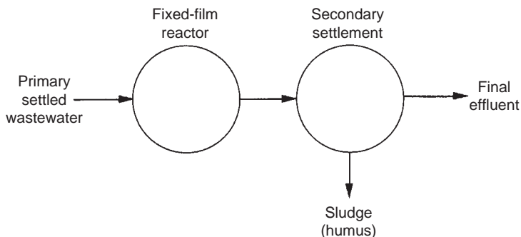
FIGURE 15.3 Schematic layout of a fixed-film reactor.
