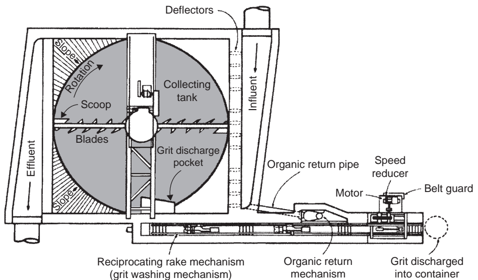
FIGURE 14.6 Outline design of a detritor or square horizontal- flow grit chamber. (Reproduced from Metcalf and Eddy (1991) with permission of McGraw-Hill, New York.)
