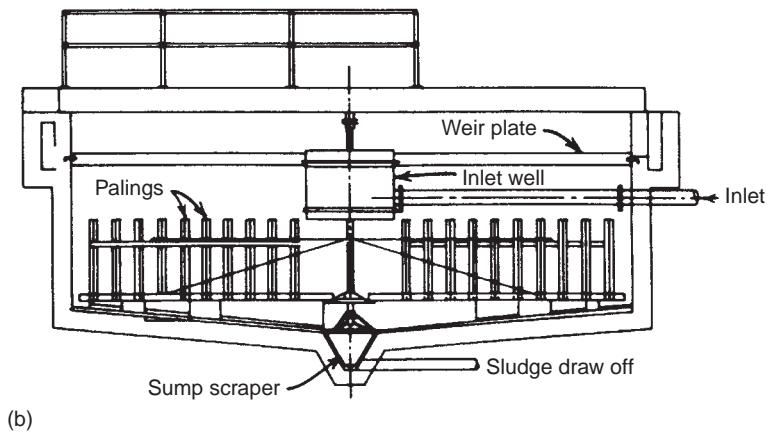
FIGURE 21.4 Picket-fence thickener in (a) plan and (b) cross-section. (Reproduced from Hammer (1977) with permission of John Wiley and Sons Inc., New York.)
