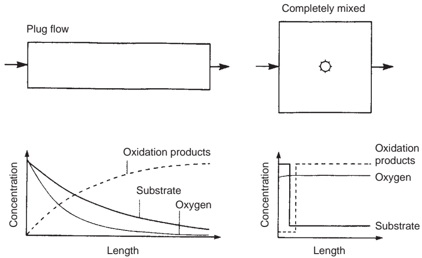
FIGURE 17.14 Comparison of the utilization of substrate and oxygen, and the production of oxidation products through a plug-flow and completely mixed reactor.
