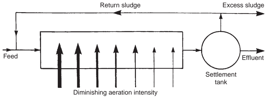
FIGURE 17.16 Schematic flow diagram of tapered aeration in a plug-flow activated sludge system.
