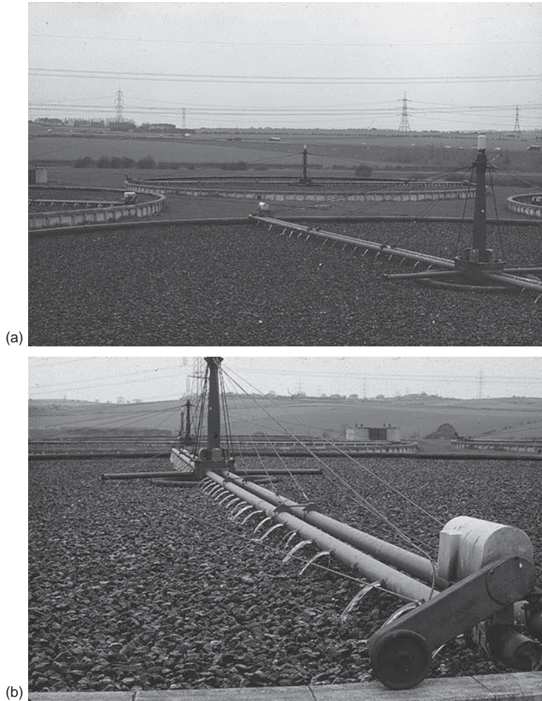
FIGURE 16.1 Standard circular percolating filters (a) showing details of the rotating distribution arm delivering settled wastewater onto the surface of the medium which is driven by a simple motorized wheel (b).
