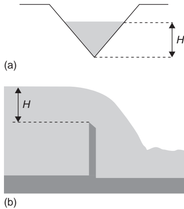
FIGURE 9.5 Sectional drawings of a 90° V-notch weir, (a) cross-section and (b) side profile through weir, where H is the vertical distance (head) between the point of the weir and the true surface of the water.
