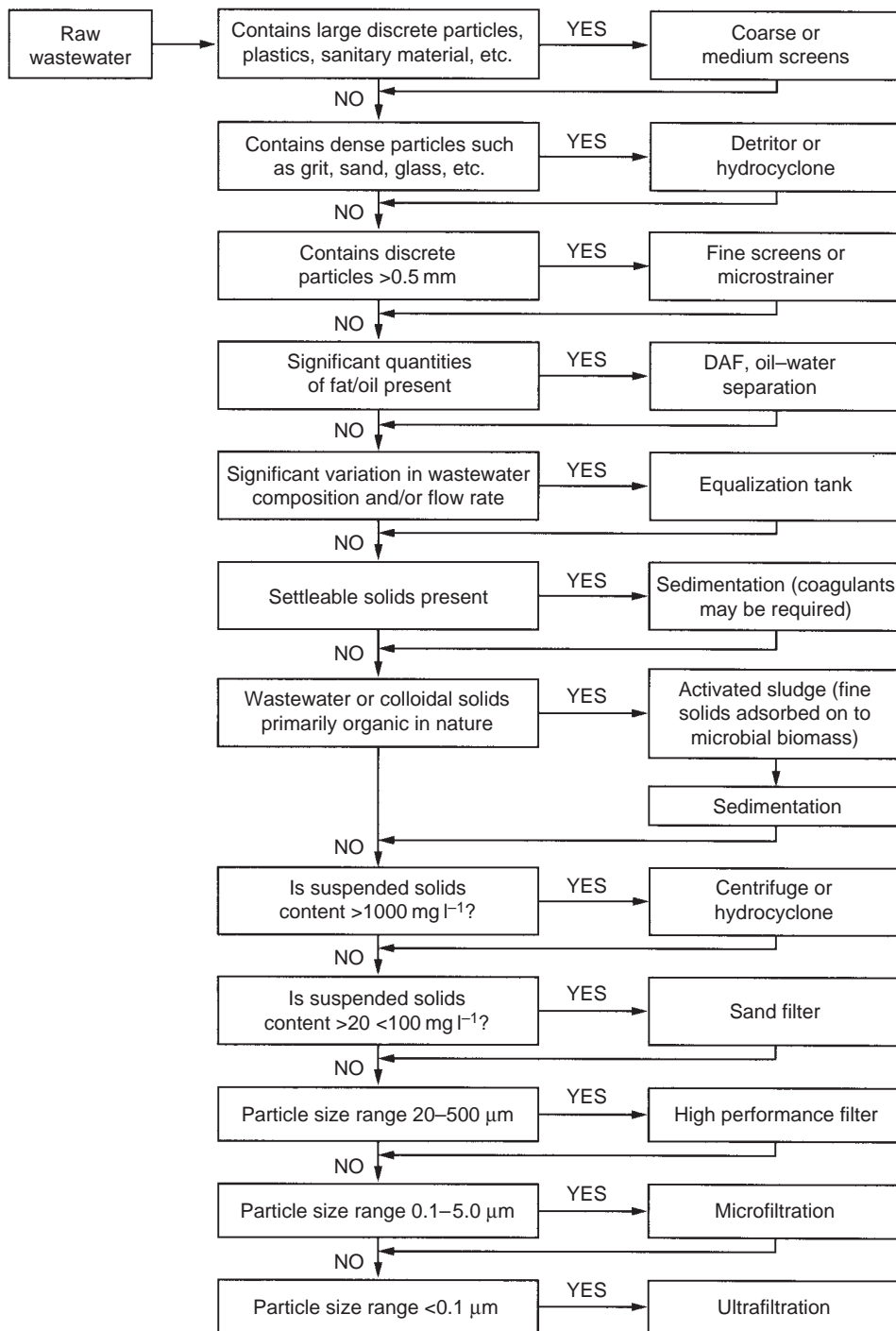
FIGURE 14.15 Process selection algorithm for solids removal in wastewater treatment.
