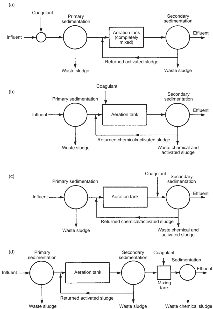
FIGURE 20.10 Phosphorus removal using coagulants. (a) Primary coagulation; (b) simultaneous coagulation; (c) post-coagulation and (d) post-precipitation.
