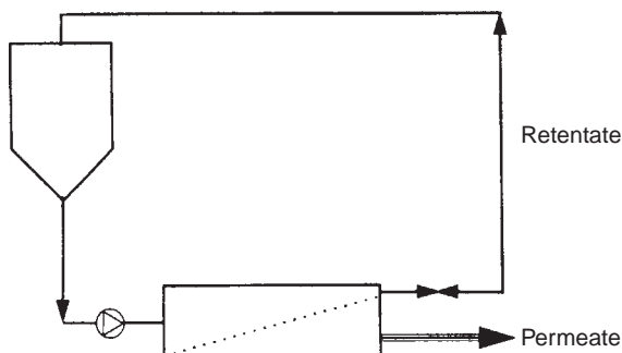
FIGURE 20.19 Schematic diagram of a simple batch plant arrangement. (Reproduced from Scott and Hughes (1996) with permission of Kluwer Academic Publishers, Dordrecht, The Netherlands.)
