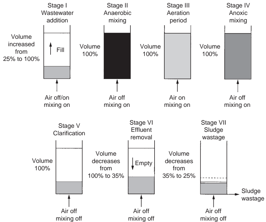
FIGURE 17.38 Sequencing batch reactor system for nutrient removal.
