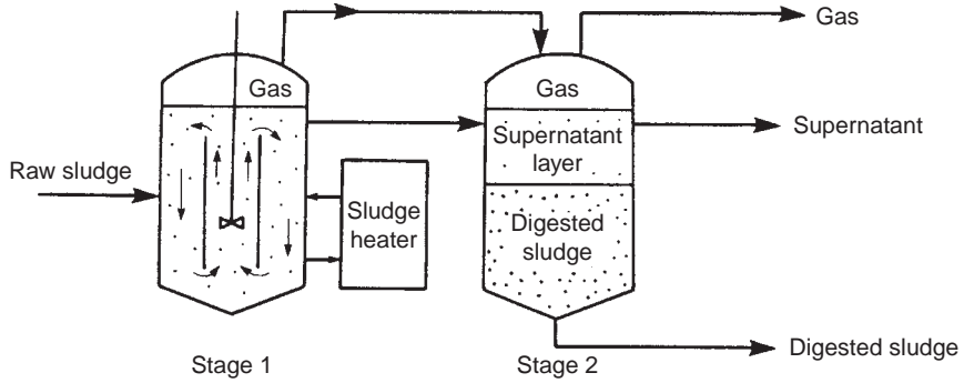
FIGURE 19.4 Two-stage anaerobic sludge digester.
