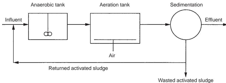
FIGURE 17.34 The two-stage (A–O) biological phosphorus removal process.
