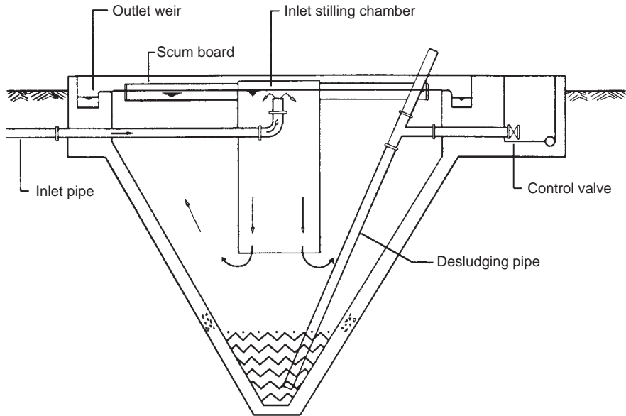
FIGURE 14.9 Upward-flow primary sedimentation tank. (Reproduced from Casey (1997) with permission of John Wiley and Sons Ltd, Chichester.)
