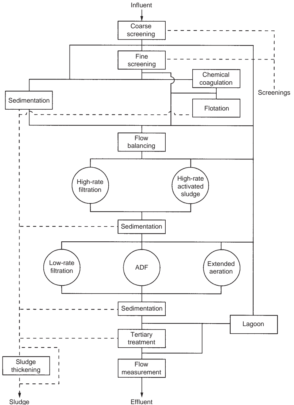
FIGURE 14.3 Summary of the main process options commonly employed at both domestic and industrial wastewater treatment plants. Not all these unit processes may be selected, but the order of their use remains the same.
