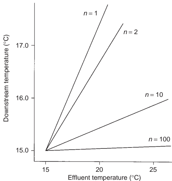
FIGURE 6.19 Effect of dilution and effluent temperature on the downstream temperature of a river with a temperature of 15^\circ\text{C} , where n is the dilution factor.
