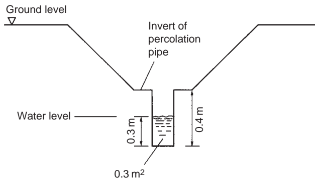
FIGURE 22.8 Irish percolation test hole dimensions.
