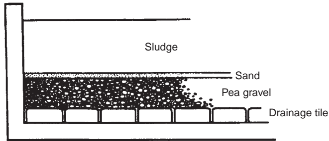
FIGURE 21.6 Cross-section through a typical sludge drying bed. (Reproduced from Institution of Water Pollution Control (1981) with permission of the Chartered Institution of Water and Environmental Management, London.)
