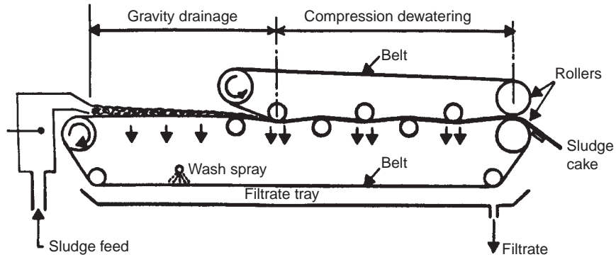
FIGURE 21.9 Schematic outline of a sludge belt press. (Reproduced from Casey and O'Connor (1980) with permission of Enterprise Ireland, Dublin.)
