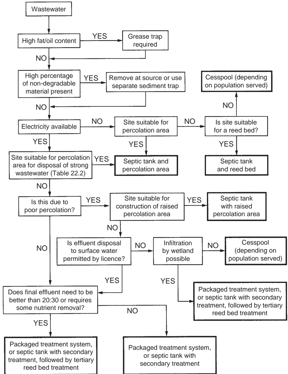
FIGURE 22.1 Process selection algorithm for small sewage treatment plants.
