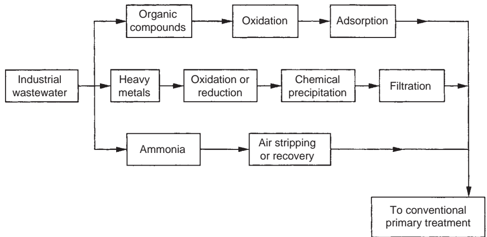
FIGURE 14.13 Main industrial pre-treatment options.
