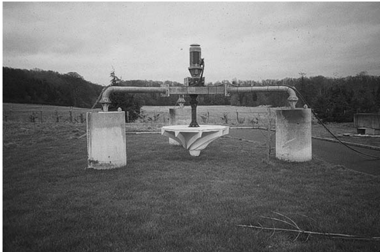
FIGURE 17.6 A vertical aerator showing the motor and gear box about to be lifted by crane into the aeration tank. This aerator is attached to three concrete floats which allow aeration to continue regardless of the depth of liquid in the aeration tank. These units are also used to keep equalization basins aerobic and can also be used to reoxygenate rivers.
