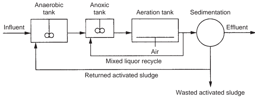
FIGURE 17.37 Schematic layout of the AAO activated sludge process.
