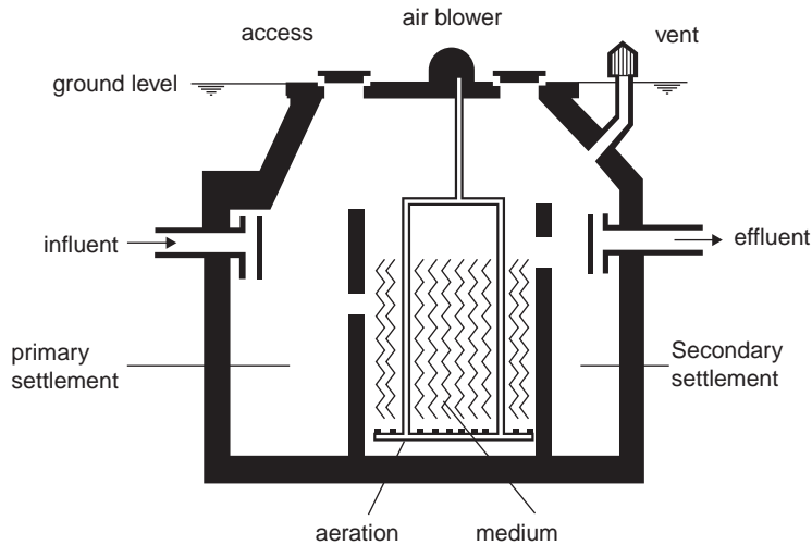
FIGURE 22.10 Schematic diagram of a biological aerated filter.
