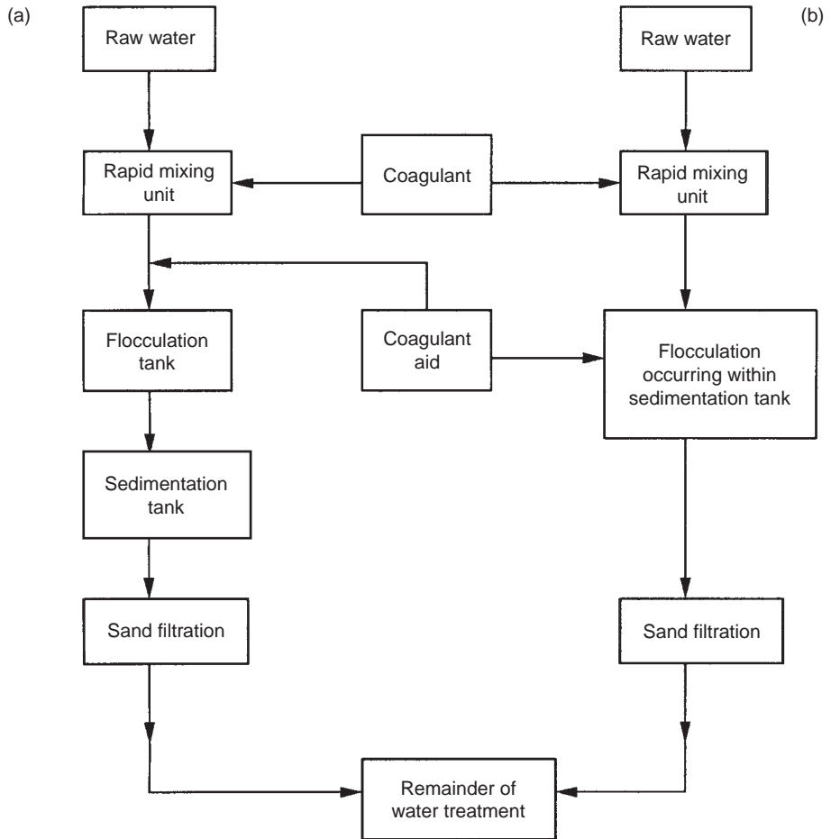
FIGURE 10.4 Different alternatives to the addition of coagulant and coagulant aids (polyelectrolytes); (a) is widely used in the USA and (b) is common practice in the UK.
