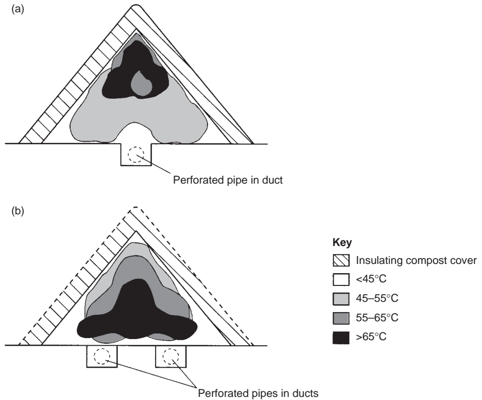
FIGURE 21.16 Temperature profile of composting sewage sludge where (a) is positive pressure (blowing) aeration and (b) negative pressure (sucking) aeration. (Reproduced from Stentiford et al. (1985) with permission of Elsevier Science Ltd, London.)
