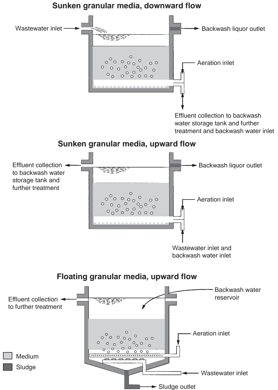
FIGURE 16.12 Commonest designs of submerged BAFs.
