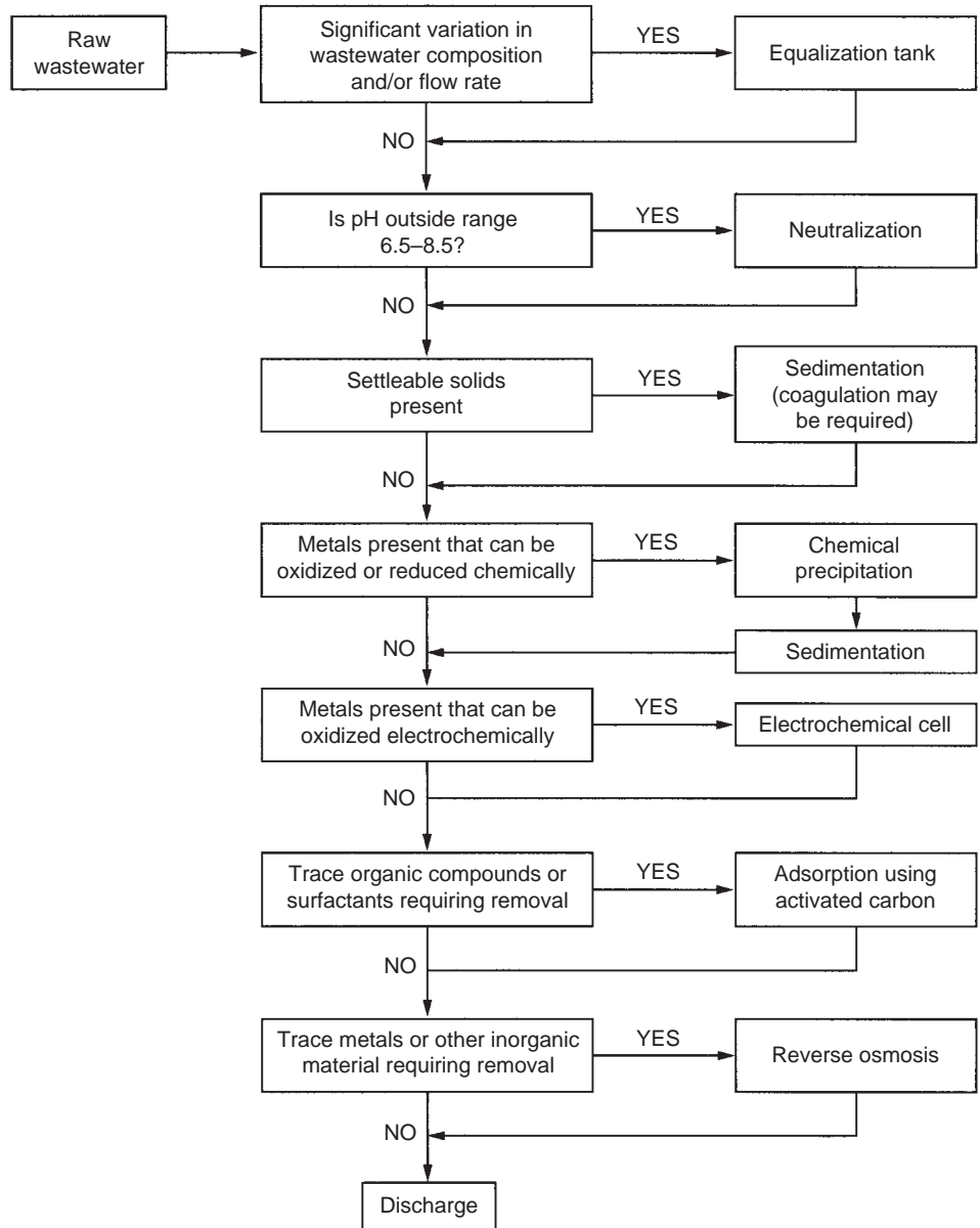
FIGURE 14.14 Process selection algorithm for physico-chemical treatment.
