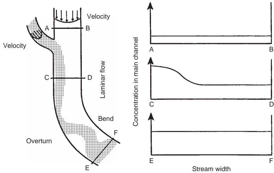
FIGURE 9.3 A tributary entering a river will not mix with the main channel flow due to the maximum velocity, which occurs in the centre of the channel pushing the influent water to the side of the river it has entered. Complete mixing will not occur until laminar flow is disrupted by either a bend in the river (overturn) or a waterfall (turbulent mixing). (Reproduced from Chapman (1996) with permission of UNESCO, Paris.)
