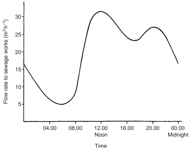
FIGURE 13.3 Example of the diurnal variation of flow to a sewage treatment plant.
