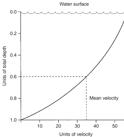
FIGURE 3.3 Relationship between depth and flow velocity. (Reproduced from Townsend (1980) with permission of Edward Arnold, London.)
