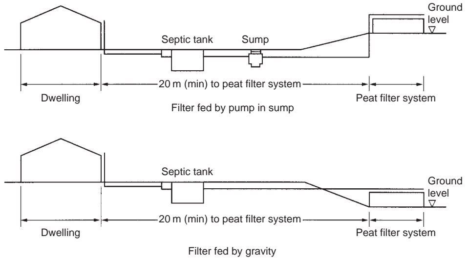
FIGURE 22.14 Layout of Puroflow® peat filter system. (Reproduced from National Standards Authority of Ireland (1991) with permission of the National Standards Authority of Ireland, Dublin.)
