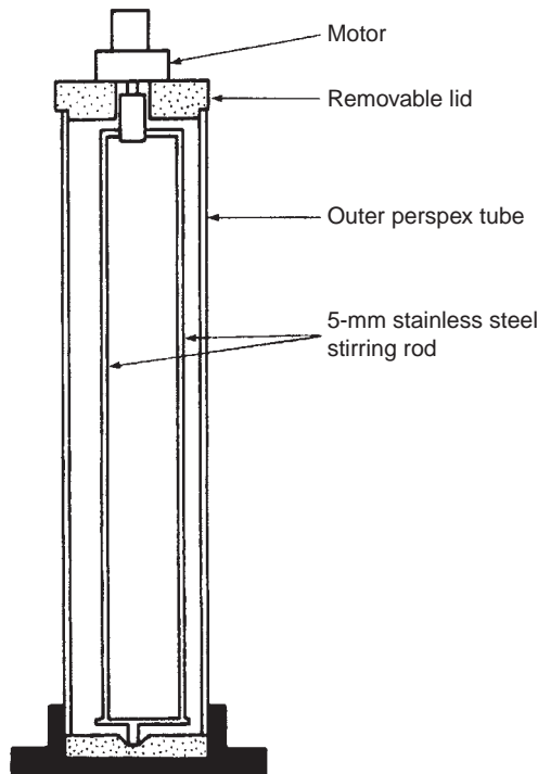
FIGURE 17.4 The standard SSVI settling apparatus developed at the Water Research Centre and available from Triton Ltd, Great Dunmow, Essex.
