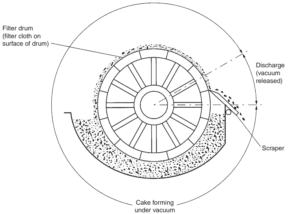
FIGURE 21.11 Principle of vacuum filtration for dewatering sludge. (Reproduced from Casey and O'Connor (1980) with permission of Enterprise Ireland, Dublin.)
