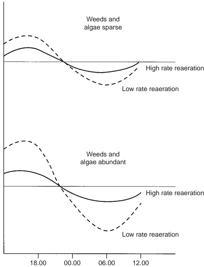
FIGURE 3.6 Diurnal variation of dissolved oxygen in rivers due to eutrophication. Difference in oxygen concentration (y-axis) at different rates of reaeration (Section 5.3) is shown.
