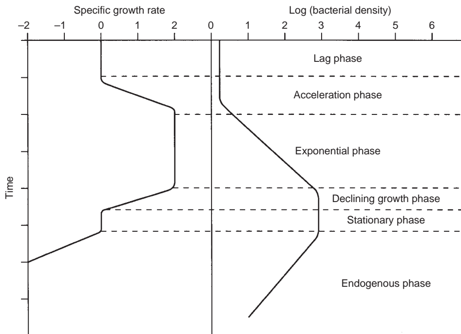
FIGURE 15.6 The microbial growth curve showing bacterial density and specific growth rate at various microbial growth phases. (Reproduced from Benefield and Randall (1980) with permission of Prentice-Hall Inc., New York.)
