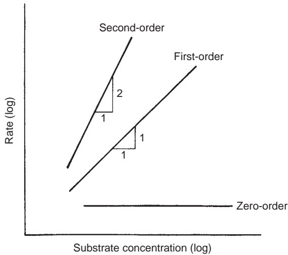
FIGURE 15.8 Log plots of reaction rates.
