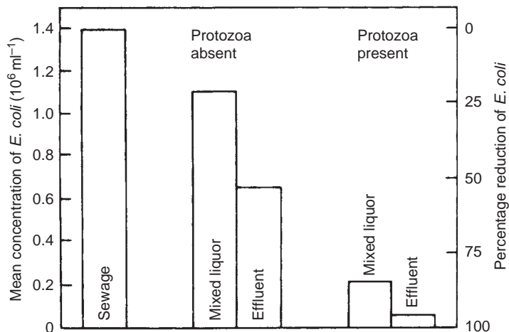
FIGURE 12.5 Removal of E. coli in experimental activated sludge plants operating in the absence or presence of ciliated protozoa. (Reproduced from Curds and Fey (1969) with permission of Elsevier Science Ltd, Oxford.)
