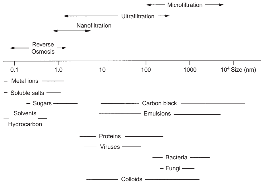
FIGURE 20.13 Application size range of membrane filtration processes. (Reproduced from Scott and Hughes (1996) with permission of Kluwer Academic Publishers, Dordrecht, The Netherlands.)
