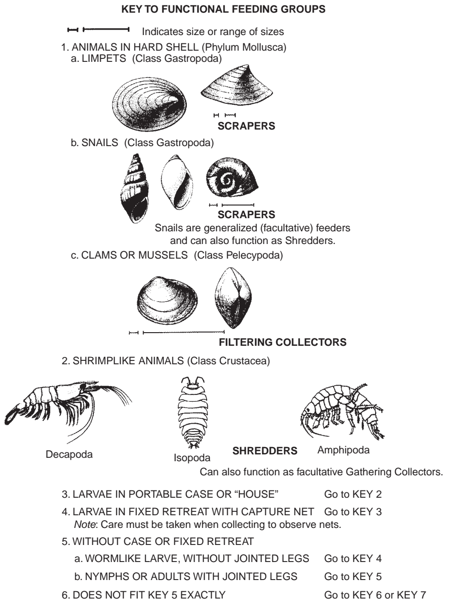
FIGURE 4.6 A simplified key to macro-invertebrate riverine functional feeding groups. (Reproduced from Merritt and Cummins (2007) with permission of Elsevier, London.)
