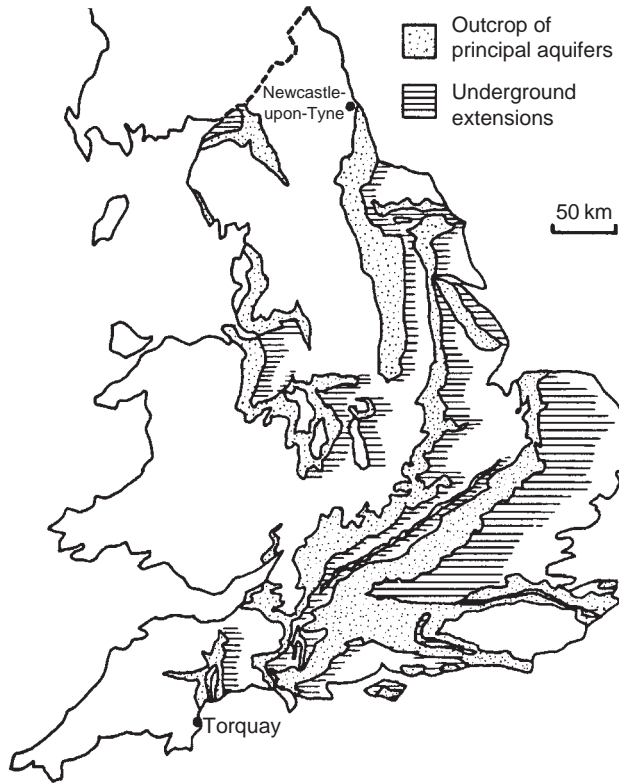
FIGURE 2.3 Location of the principal aquifers in England and Wales. (Reproduced from Open University (1974) with permission of the Open University Press, Milton Keynes.)
