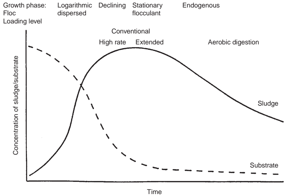
FIGURE 17.2 The microbial growth curve showing the operational growth phase used in different modes of activated sludge.
