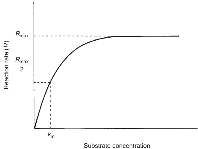
FIGURE 15.12 The rate of enzyme-catalysed reactions as presented by the Michaelis–Menten equation.
