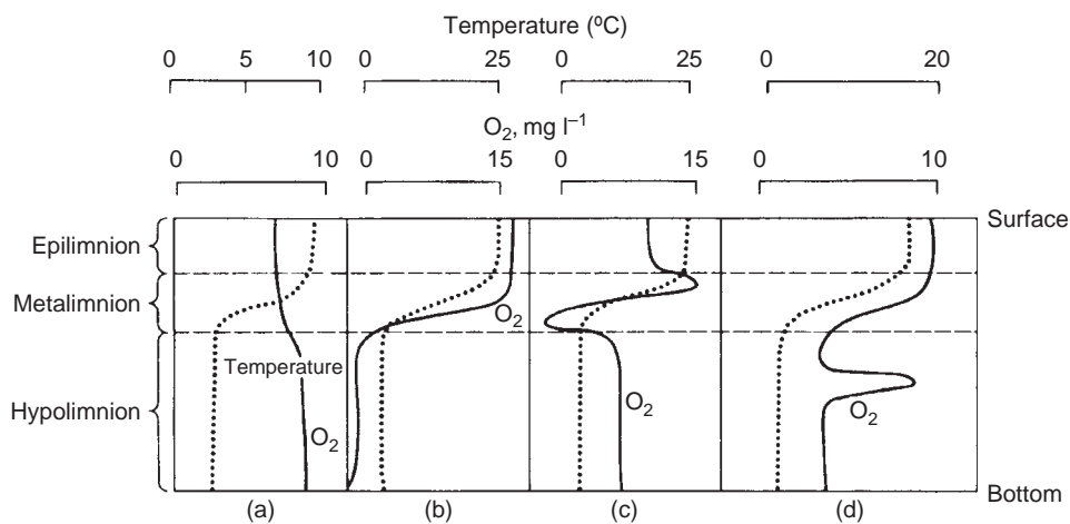
FIGURE 3.10 Types of oxygen distribution with depth. (a) Orthograde curve typical of an unproductive lake. (b) Clinograde curve from a productive lake. (c) Positive and negative heterograde curves. Here photosynthesis from a layer of algae just above the thermocline raises oxygen concentration in the upper part of the metalimnion. Respiration occurring during bacterial decomposition and zooplankton grazing lowers oxygen levels just below the thermocline (metalimnion minimum). (d) Anomalous curves due to the inflow of dense, cool, oxygen-rich stream inflows, which form a discrete layer. In this example, the oxygen-rich stream inflow is in midhypolimnion. (Reproduced from Horne and Goldman (1994) with permission of McGraw-Hill, New York.)
