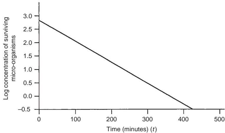
FIGURE 12.6 Destruction of pathogens according to Chick's law.
