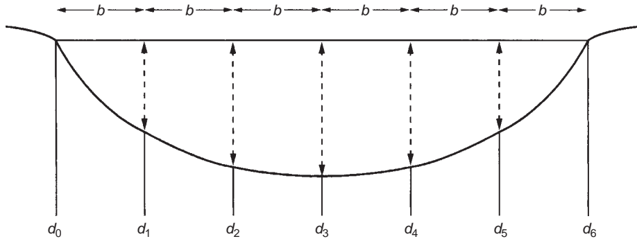
FIGURE 9.4 In order to calculate river discharge rate by current metering, river channels are split into separate panels of width ( b ) with the depth ( d ) and the flow velocity ( v ) measured at the boundary of each panel.
