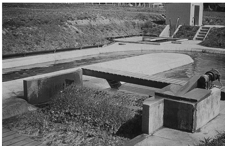
FIGURE 17.8 An oxidation ditch using a horizontal rotor.
