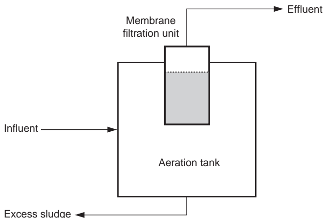
FIGURE 20.22 MBR system employing an internal membrane filtration unit.
