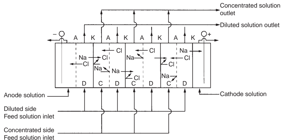
FIGURE 20.24 A typical electrodesalination cell. A: anion-exchange membrane; K: cation-exchange membrane. (Reproduced from Scott and Hughes (1996) with permission of Kluwer Academic Publishers, Dordrecht, The Netherlands.)
