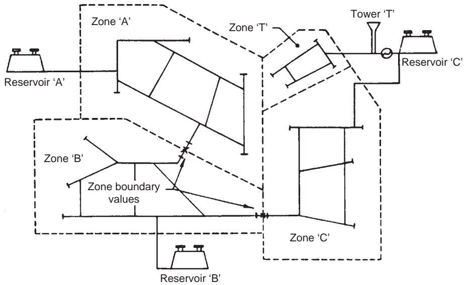
FIGURE 10.12 Schematic diagram showing that water distribution networks are broken down into operational zones each supplied by a service reservoir. (Reproduced from Latham (1990) with permission of the Chartered Institution of Water and Environmental Management, London.)
