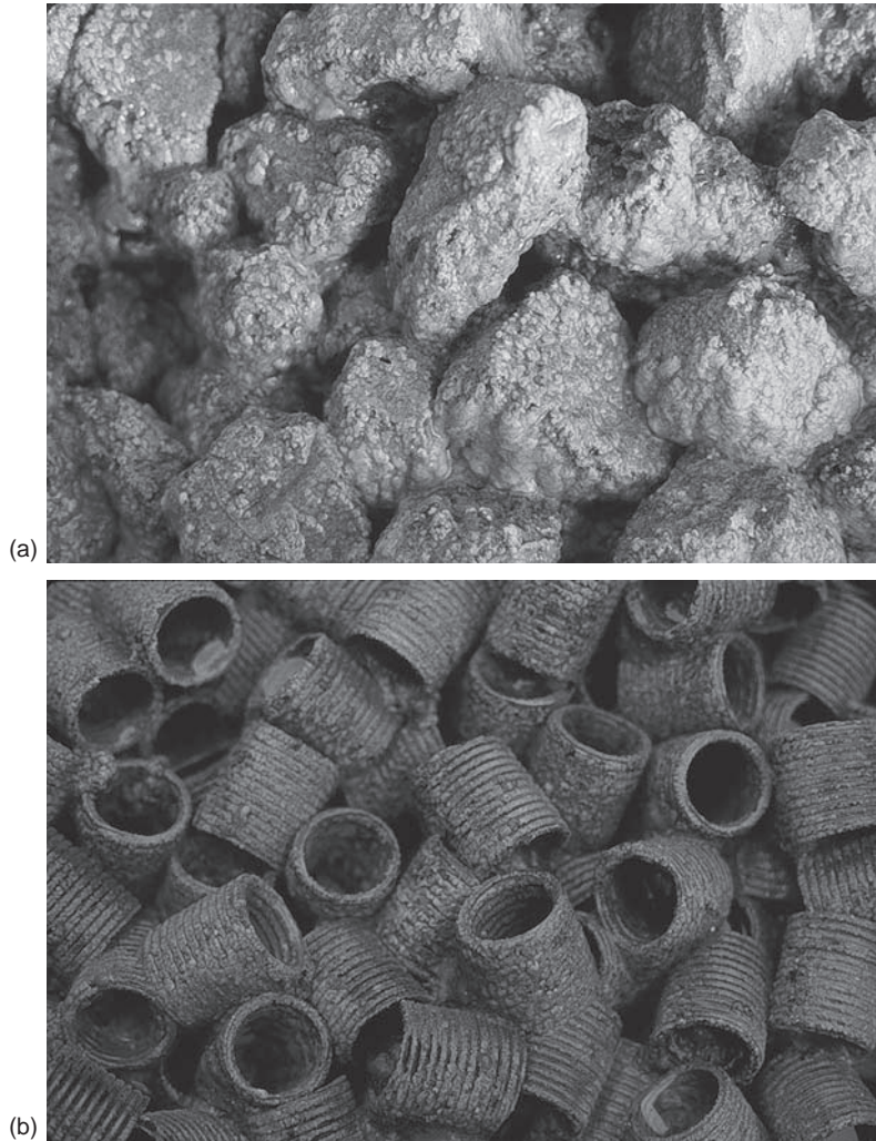
FIGURE 16.7 Percolating filter medium covered with biofilm (a) 50 mm blast furnace slag and (b) Flocor RC a 50 mm random plastic filter medium.
