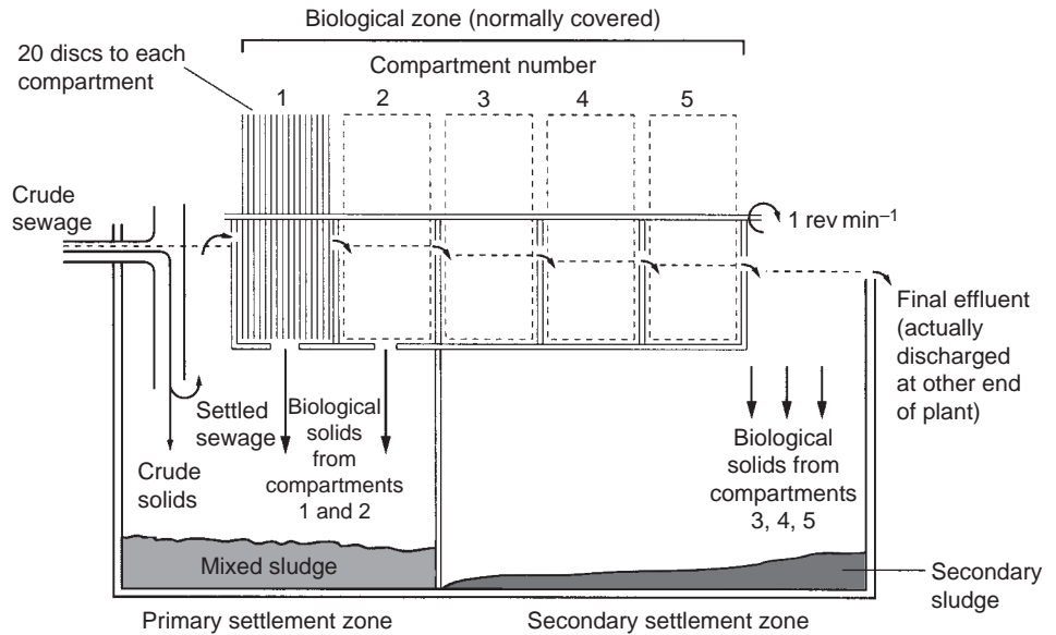
FIGURE 16.10 Rotating biological contractor. (Reproduced from Mann (1979) with permission of WRc plc, Medmenham.)
