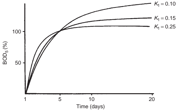
FIGURE 5.8 The effect of various rate constants in the calculation of the same BOD. The result is expressed as a percentage. (Reproduced from Tebbutt (1992) with permission of Butterworth-Heinemann Ltd, Oxford.)
