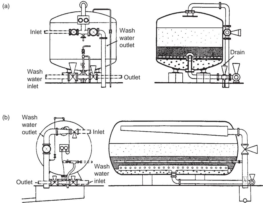
FIGURE 10.9 Schematic layout of (a) a vertical pressure water filter and (b) a horizontal pressure filter. (Reproduced from Solt and Shirley (1991) with permission of Ashgate Publishing Ltd, Aldershot.)
