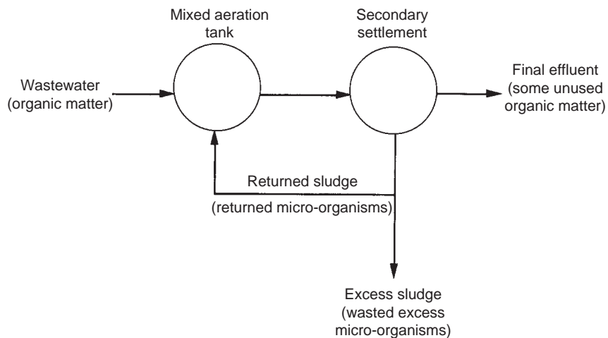
FIGURE 15.4 Schematic for a completely mixed (activated sludge) reactor.
