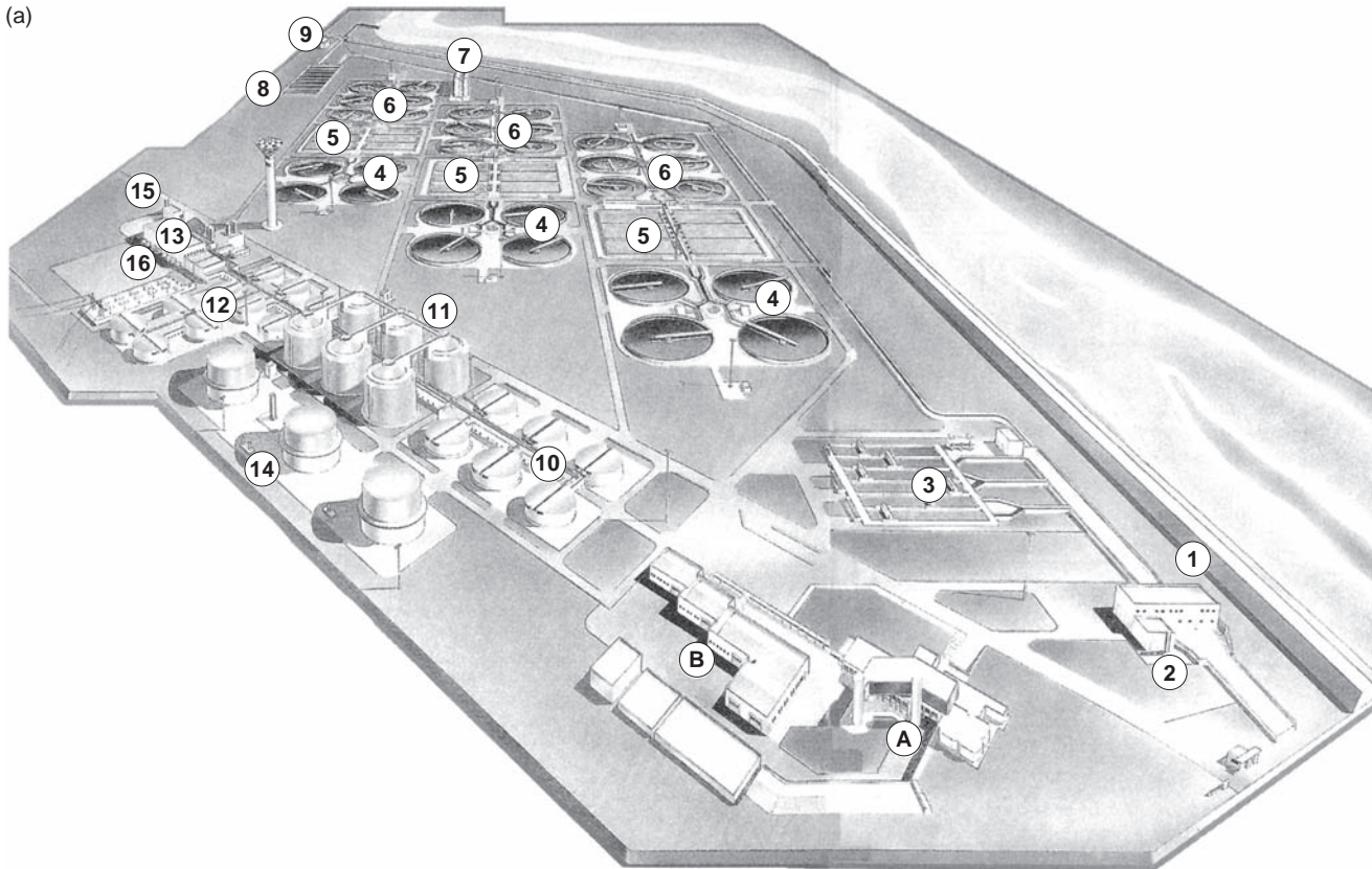
FIGURE 14.18 The Po-Sangone wastewater treatment plant in Torino, Italy. (a) Plan layout of plant, (b) water process flow diagrams and (c) sludge process flow diagram. Wastewater treatment : 1. storm water overflow; 2. screening; 3. grit removal; 4. primary sedimentation; 5. aeration tanks; 6. secondary sedimentation; 7. emergency chlorination; 8. filtration; 9. effluent outfall. Sludge treatment : 10. raw sludge thickeners; 11. digestion tanks; 12. digested sludge thickeners; 13. power house; 14. biogas storage; 15. filter press house; 16. transformer station. A and B are administrative areas. (Reproduced by permission of Ing. Paolo Romano, General Manager, Azienda Po Sangone.)
