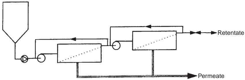
FIGURE 20.20 Schematic diagram of a feed and bleed plant. (Reproduced from Scott and Hughes (1996) with permission of Kluwer Academic Publishers, Dordrecht, The Netherlands.)
