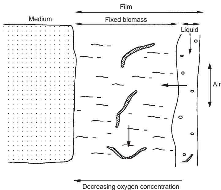
FIGURE 16.4 Diagrammatic representation of the structure of film in a fixed-film reactor.
