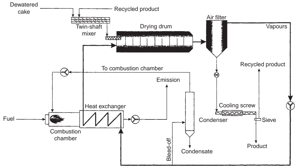
FIGURE 21.5 Schematic process flow diagram for the thermal drying of digested sludge. (Reproduced from CIWEM (1999) with permission of the Chartered Institution of Water and Environmental Management, London.)
