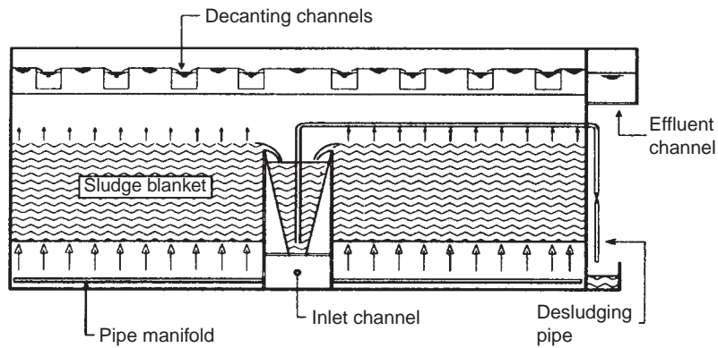
FIGURE 10.6 Schematic layout of a flat-bottomed sludge-blanket clarifier. (Reproduced from Casey (1997) with permission of John Wiley and Sons Ltd, Chichester.)
