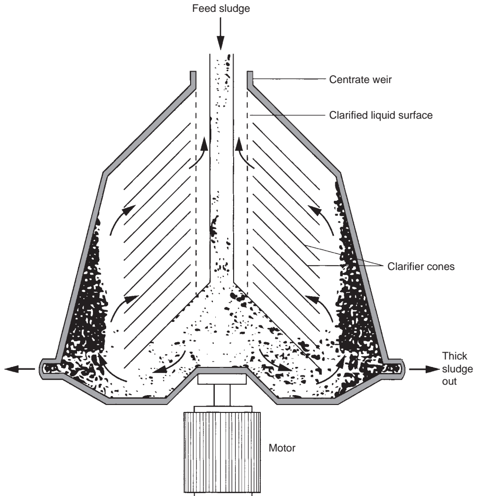
FIGURE 21.12 Schematic diagram of a nozzle-bowl centrifuge for dewatering sludge. (Reproduced from Institution of Water Pollution Control (1981) with permission of the Chartered Institution of Water and Environmental Management, London.)
