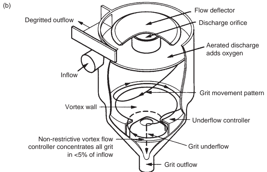
FIGURE 14.5 Grit separation using vortex-type systems: (a) a Pista grit separator manufactured by Smith and Loveless Ltd and (b) a teacup unit manufactured by Eutek Ltd. (Reproduced from Metcalf and Eddy (1991) with permission of McGraw-Hill, New York.)
