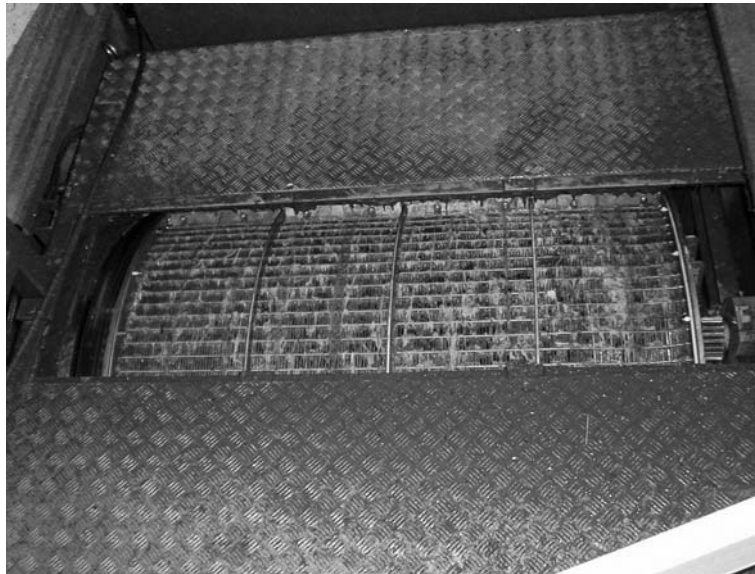
FIGURE 14.4 Rotary drum screen. These can be difficult to maintain due to becoming blocked with fibres from sanitary products.
