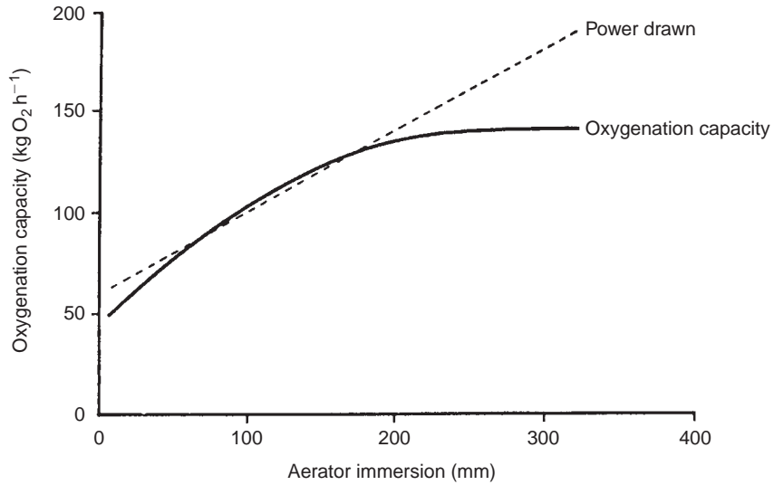
FIGURE 17.11 The oxygenation capacity (OC) and power used by a cone aerator at various depths of immersion.
