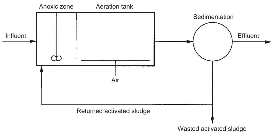
FIGURE 17.31 Schematic layout of a conventional pre-nitrification system.
