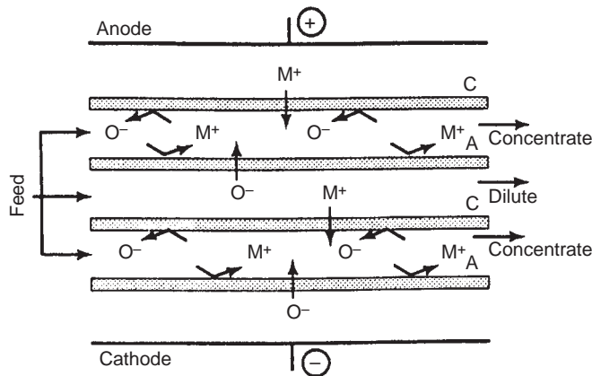
FIGURE 20.23 Separation by an electrodesalination cell. C: cation transfer membrane; A: anion transfer membrane. (Reproduced from Scott and Hughes (1996) with permission of Kluwer Academic Publishers, Dordrecht, The Netherlands.)
