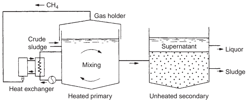
FIGURE 19.5 Conventional sludge digestion plant. (Reproduced from Tebbutt (1992) with permission of Butterworth- Heinemann Ltd, Oxford.)
