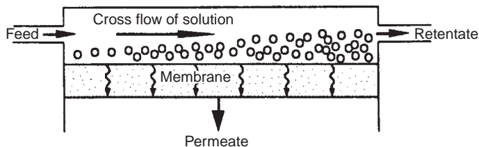
FIGURE 20.16 Cross-flow membrane separations. (Reproduced from Scott and Hughes (1996) with permission of Kluwer Academic Publishers, Dordrecht, The Netherlands.)
